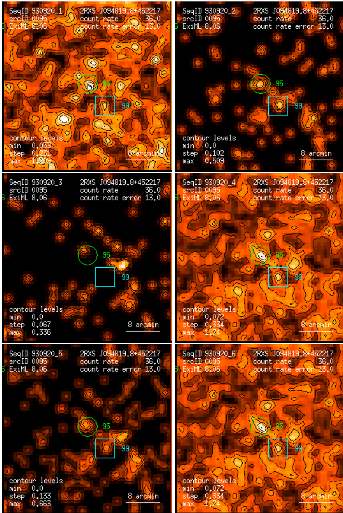
Figure 95: RASS 930920: detection 0095: band rate images, Gaussian filter: (1) PSPC channels 11 – 41, (2) 52 – 90, (3) 91 – 201, (4) 11 – 235, (5) 52 – 201, (6) 11 – 201. Broad band rates in counts/ks. Band rate contour levels in counts/ks/arcmin 2 .
