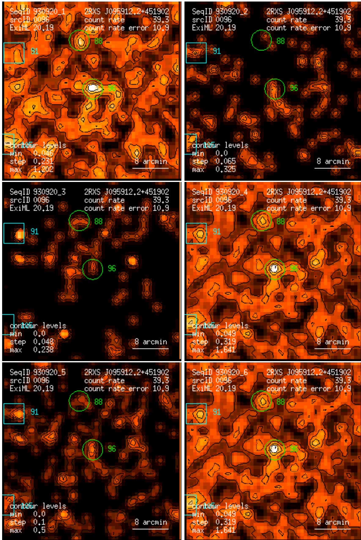
Figure 96: RASS 930920: detection 0096: band rate images, Gaussian filter: (1) PSPC channels 11 – 41, (2) 52 – 90, (3) 91 – 201, (4) 11 – 235, (5) 52 – 201, (6) 11 – 201. Broad band rates in counts/ks. Band rate contour levels in counts/ks/arcmin 2 .
