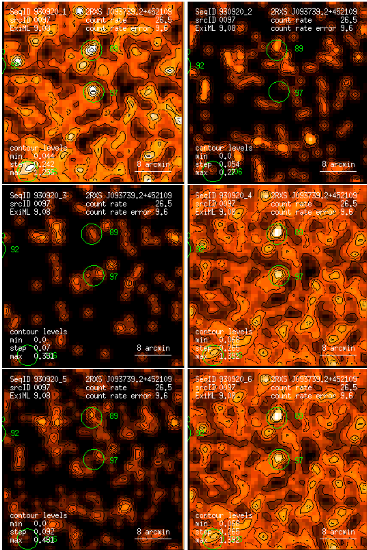
Figure 97: RASS 930920: detection 0097: band rate images, Gaussian filter: (1) PSPC channels 11 – 41, (2) 52 – 90, (3) 91 – 201, (4) 11 – 235, (5) 52 – 201, (6) 11 – 201. Broad band rates in counts/ks. Band rate contour levels in counts/ks/arcmin 2 .
