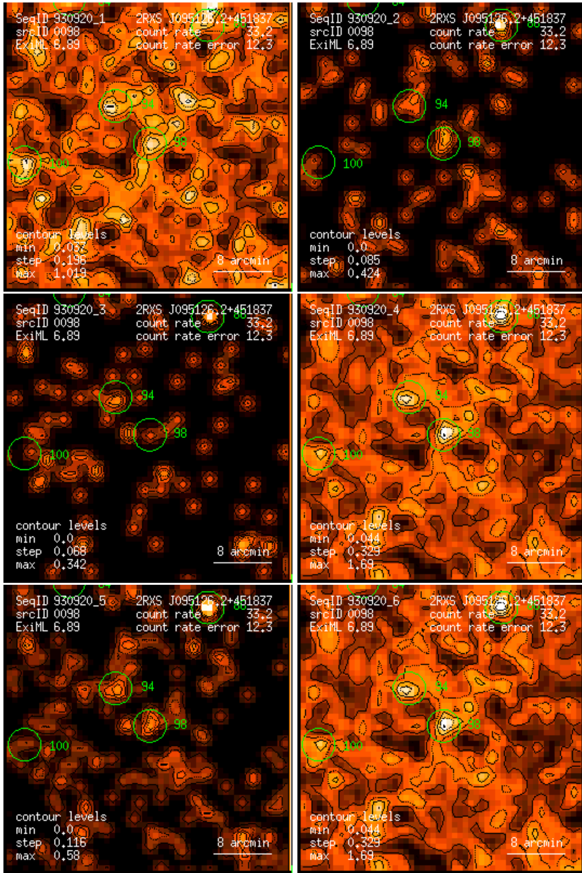
Figure 98: RASS 930920: detection 0098: band rate images, Gaussian filter: (1) PSPC channels 11 – 41, (2) 52 – 90, (3) 91 – 201, (4) 11 – 235, (5) 52 – 201, (6) 11 – 201. Broad band rates in counts/ks. Band rate contour levels in counts/ks/arcmin 2 .
