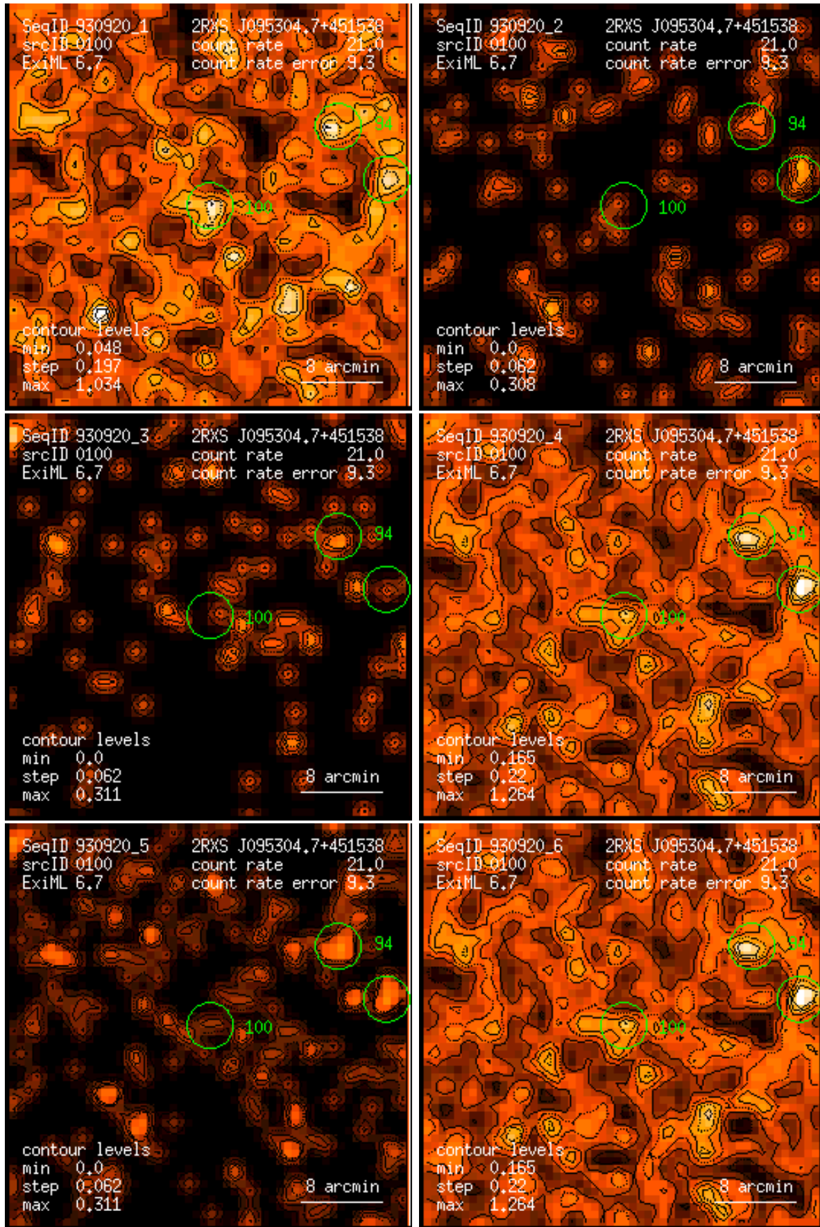
Figure 100: RASS 930920: detection 0100: band rate images, Gaussian filter: (1) PSPC channels 11 – 41, (2) 52 – 90, (3) 91 – 201, (4) 11 – 235, (5) 52 – 201, (6) 11 – 201. Broad band rates in counts/ks. Band rate contour levels in counts/ks/arcmin 2 .
