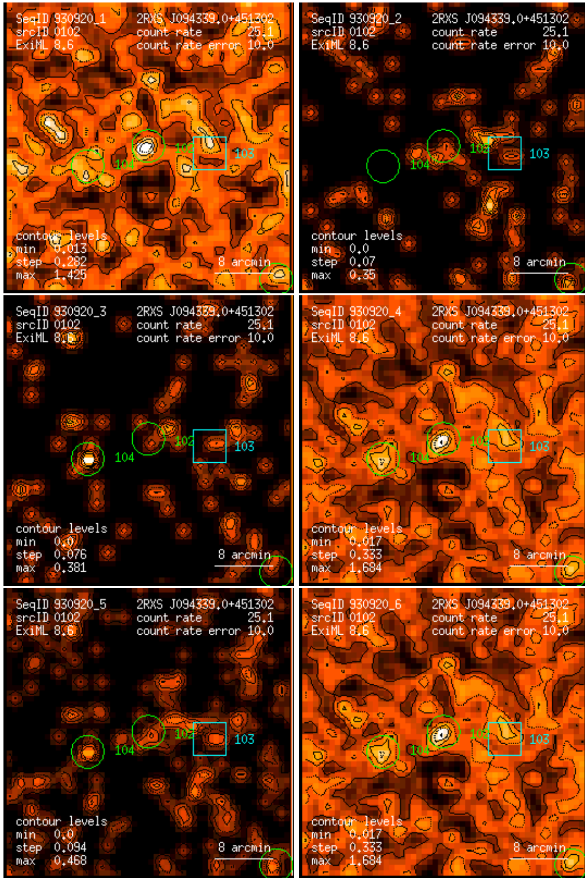
Figure 102: RASS 930920: detection 0102: band rate images, Gaussian filter: (1) PSPC channels 11 – 41, (2) 52 – 90, (3) 91 – 201, (4) 11 – 235, (5) 52 – 201, (6) 11 – 201. Broad band rates in counts/ks. Band rate contour levels in counts/ks/arcmin 2 .
