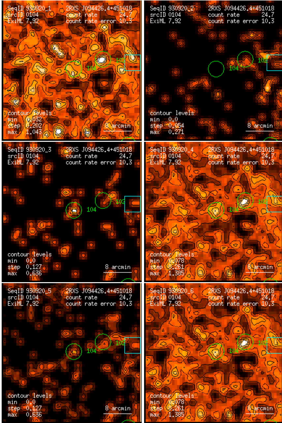
Figure 104: RASS 930920: detection 0104: band rate images, Gaussian filter: (1) PSPC channels 11 – 41, (2) 52 – 90, (3) 91 – 201, (4) 11 – 235, (5) 52 – 201, (6) 11 – 201. Broad band rates in counts/ks. Band rate contour levels in counts/ks/arcmin 2 .
