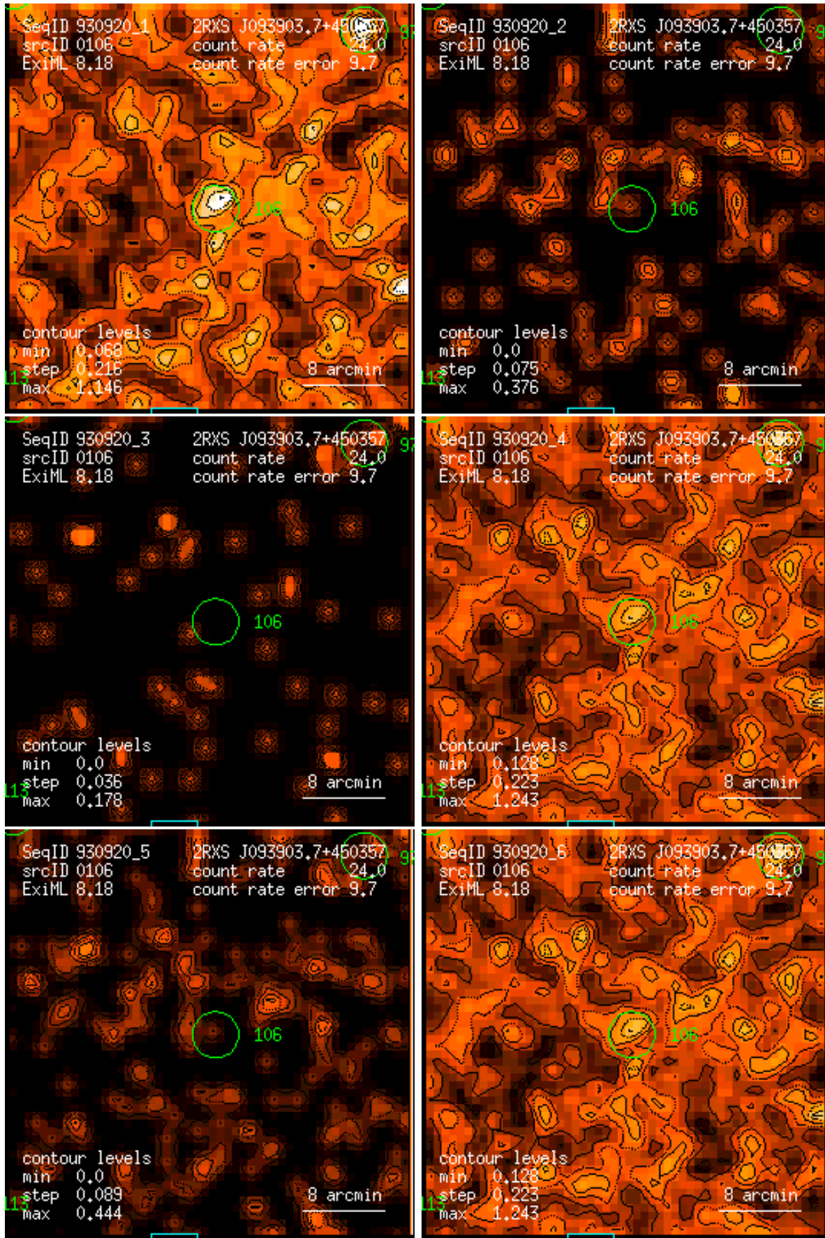
Figure 106: RASS 930920: detection 0106: band rate images, Gaussian filter: (1) PSPC channels 11 – 41, (2) 52 – 90, (3) 91 – 201, (4) 11 – 235, (5) 52 – 201, (6) 11 – 201. Broad band rates in counts/ks. Band rate contour levels in counts/ks/arcmin 2 .
