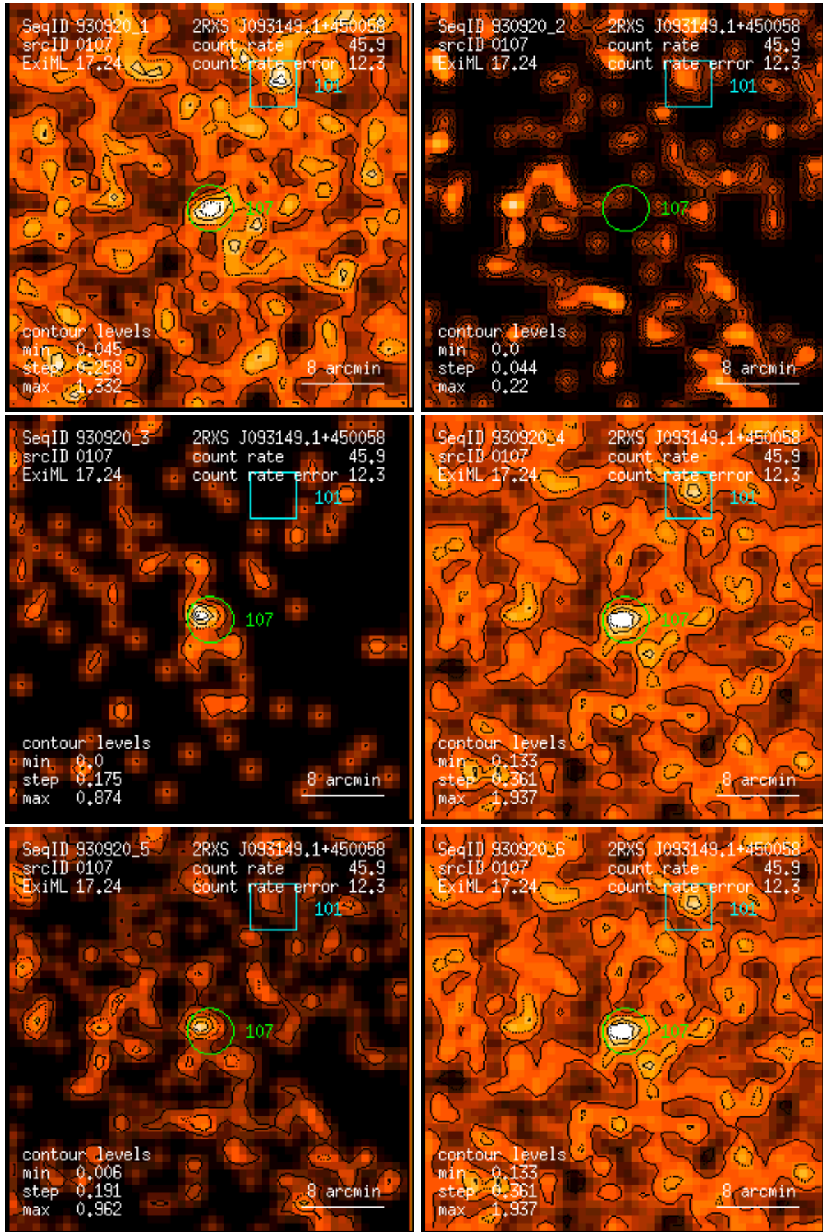
Figure 107: RASS 930920: detection 0107: band rate images, Gaussian filter: (1) PSPC channels 11 – 41, (2) 52 – 90, (3) 91 – 201, (4) 11 – 235, (5) 52 – 201, (6) 11 – 201. Broad band rates in counts/ks. Band rate contour levels in counts/ks/arcmin 2 .
