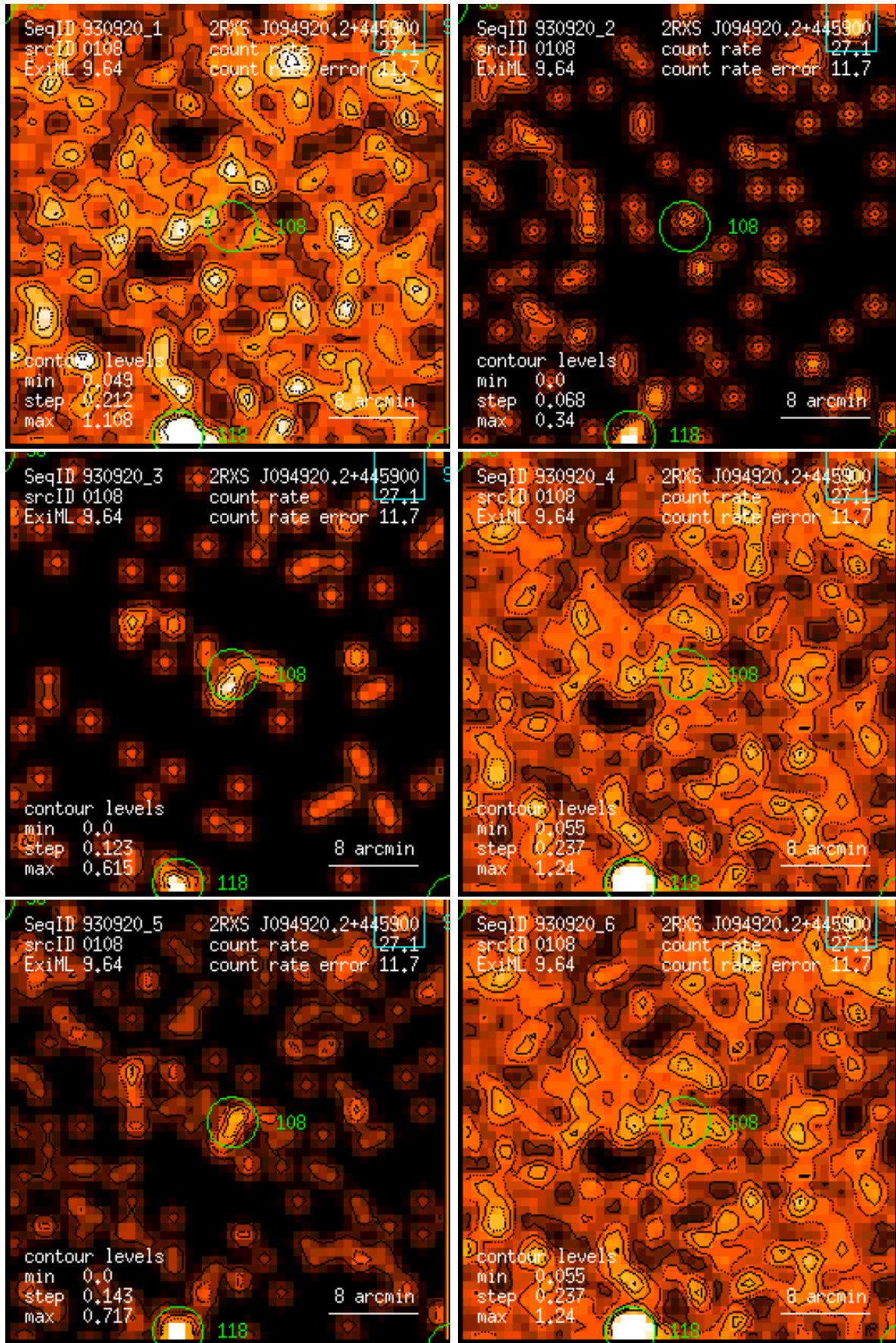
Figure 108: RASS 930920: detection 0108: band rate images, Gaussian filter: (1) PSPC channels 11 – 41, (2) 52 – 90, (3) 91 – 201, (4) 11 – 235, (5) 52 – 201, (6) 11 – 201. Broad band rates in counts/ks. Band rate contour levels in counts/ks/arcmin 2 .
