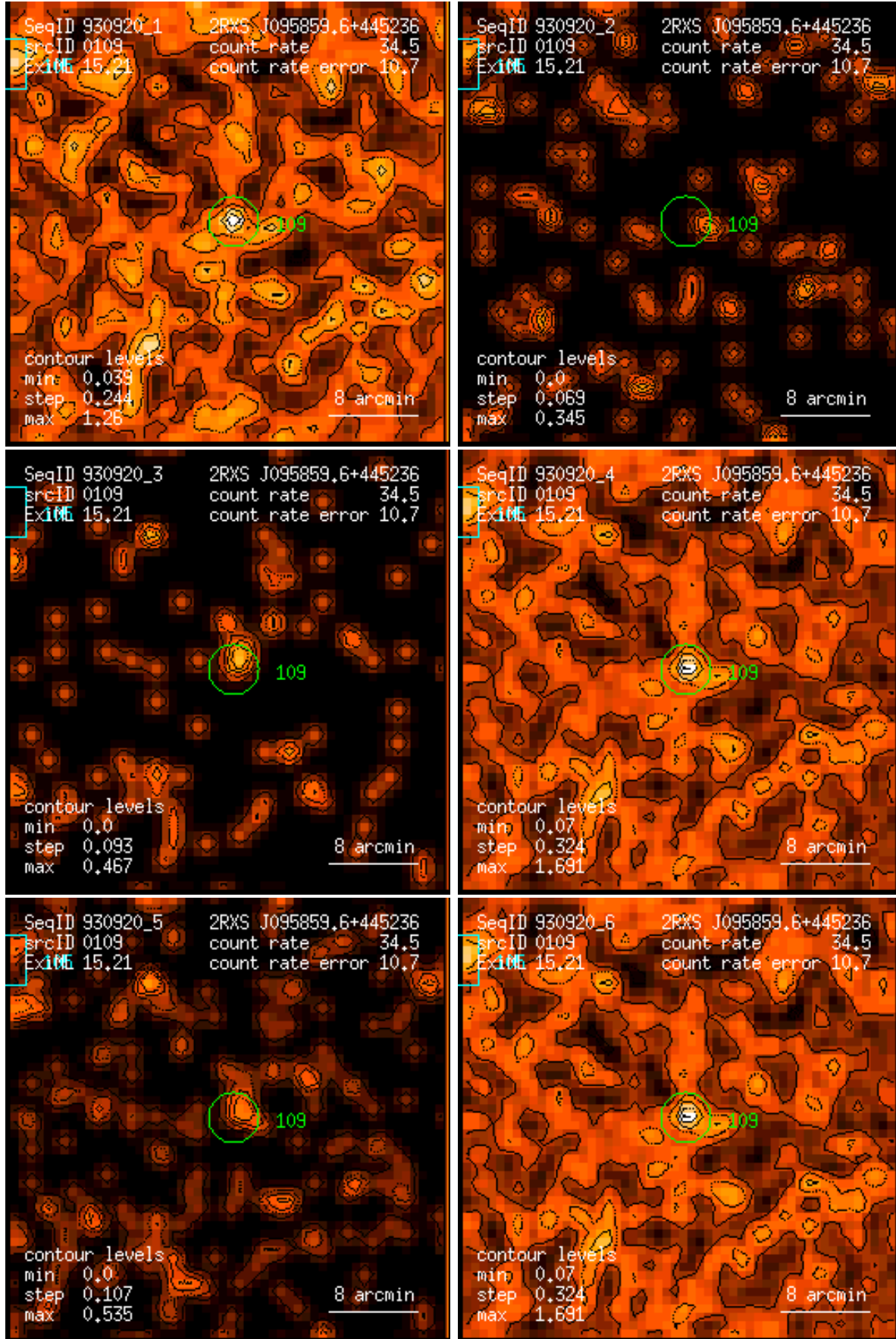
Figure 109: RASS 930920: detection 0109: band rate images, Gaussian filter: (1) PSPC channels 11 – 41, (2) 52 – 90, (3) 91 – 201, (4) 11 – 235, (5) 52 – 201, (6) 11 – 201. Broad band rates in counts/ks. Band rate contour levels in counts/ks/arcmin 2 .
