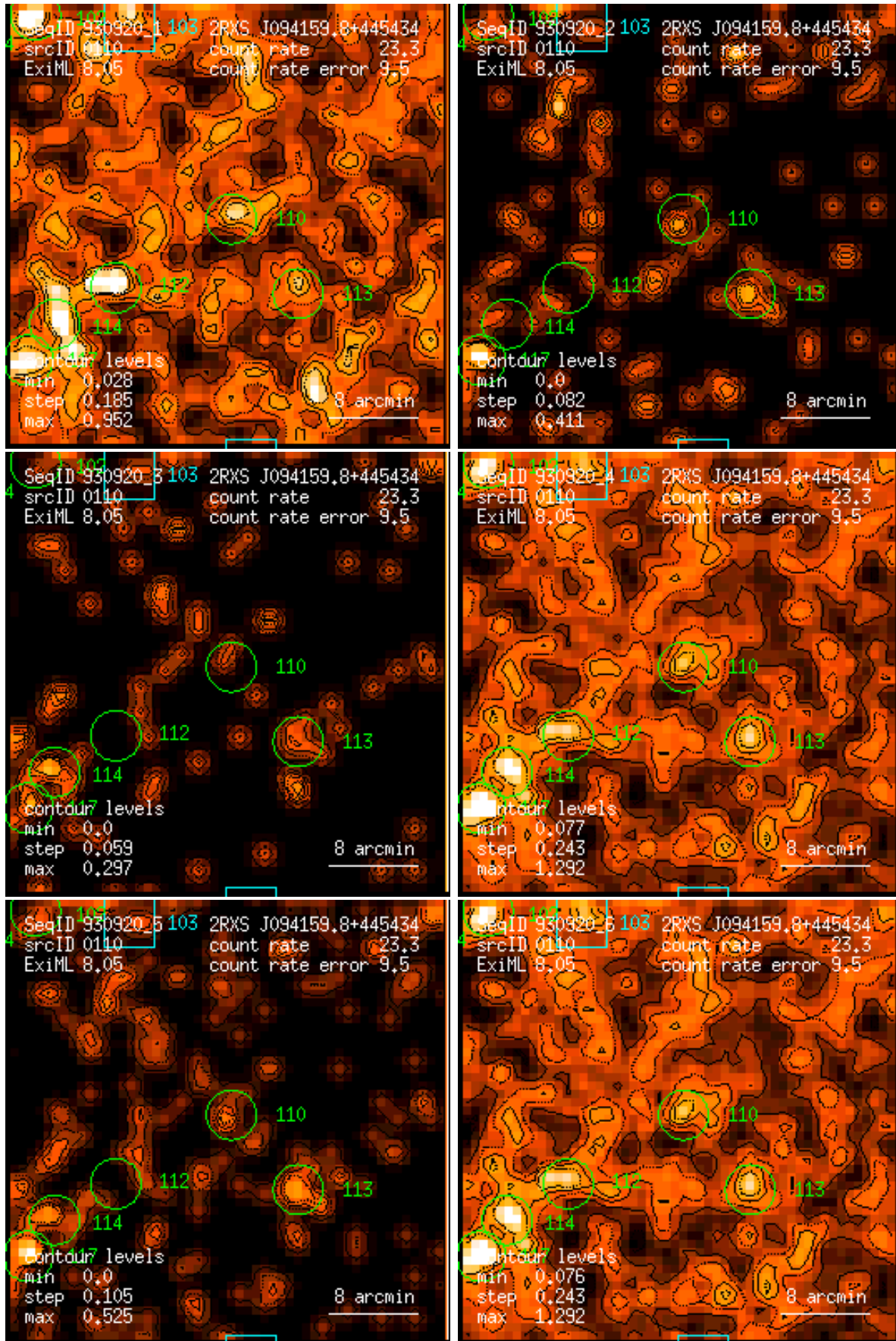
Figure 110: RASS 930920: detection 0110: band rate images, Gaussian filter: (1) PSPC channels 11 – 41, (2) 52 – 90, (3) 91 – 201, (4) 11 – 235, (5) 52 – 201, (6) 11 – 201. Broad band rates in counts/ks. Band rate contour levels in counts/ks/arcmin 2 .
