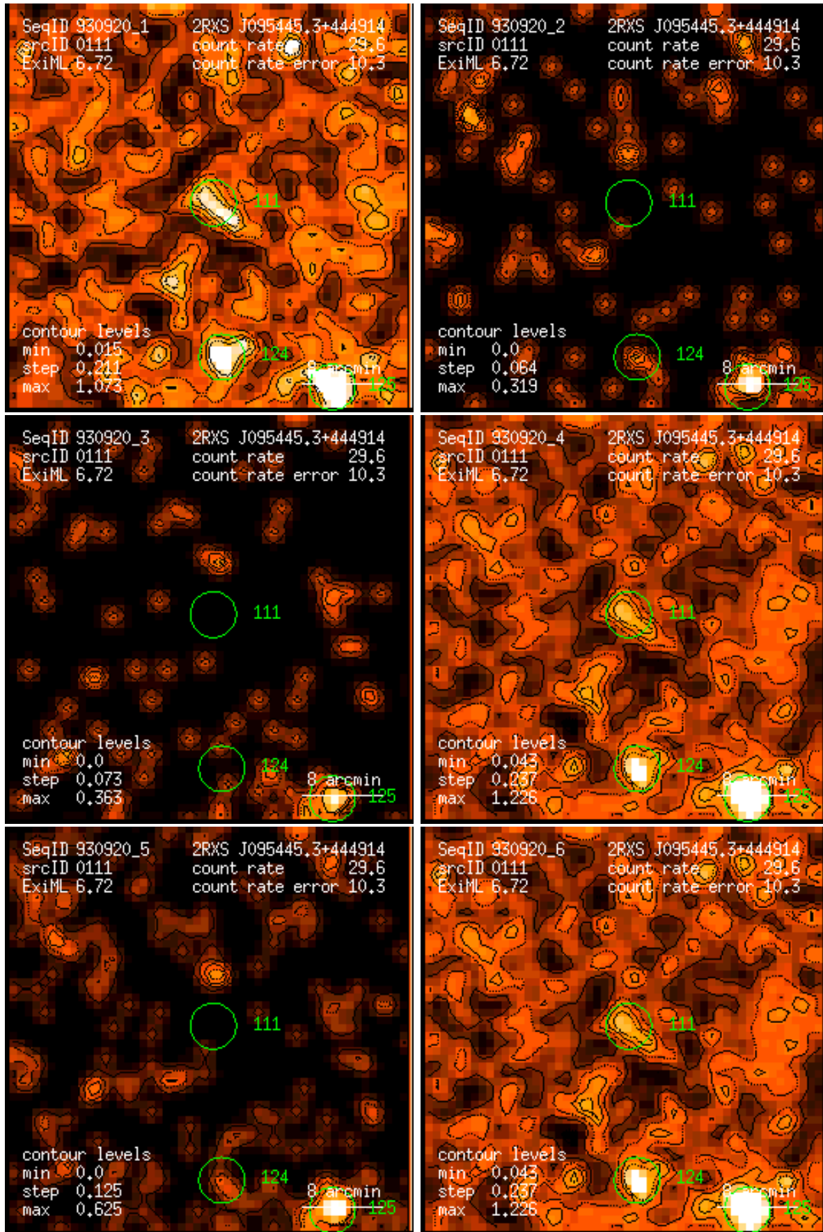
Figure 111: RASS 930920: detection 0111: band rate images, Gaussian filter: (1) PSPC channels 11 – 41, (2) 52 – 90, (3) 91 – 201, (4) 11 – 235, (5) 52 – 201, (6) 11 – 201. Broad band rates in counts/ks. Band rate contour levels in counts/ks/arcmin 2 .
