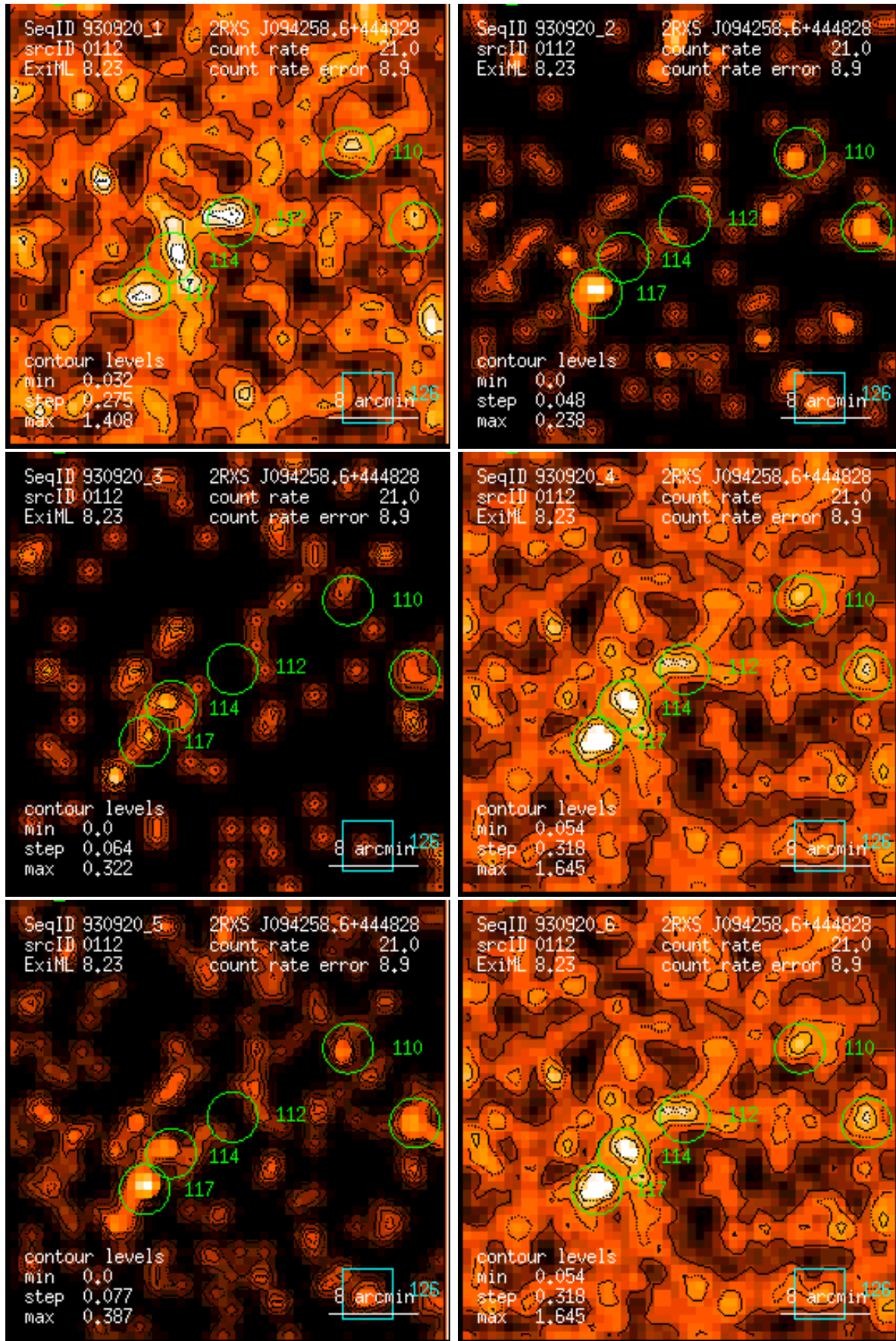
Figure 112: RASS 930920: detection 0112: band rate images, Gaussian filter: (1) PSPC channels 11 – 41, (2) 52 – 90, (3) 91 – 201, (4) 11 – 235, (5) 52 – 201, (6) 11 – 201. Broad band rates in counts/ks. Band rate contour levels in counts/ks/arcmin 2 .
