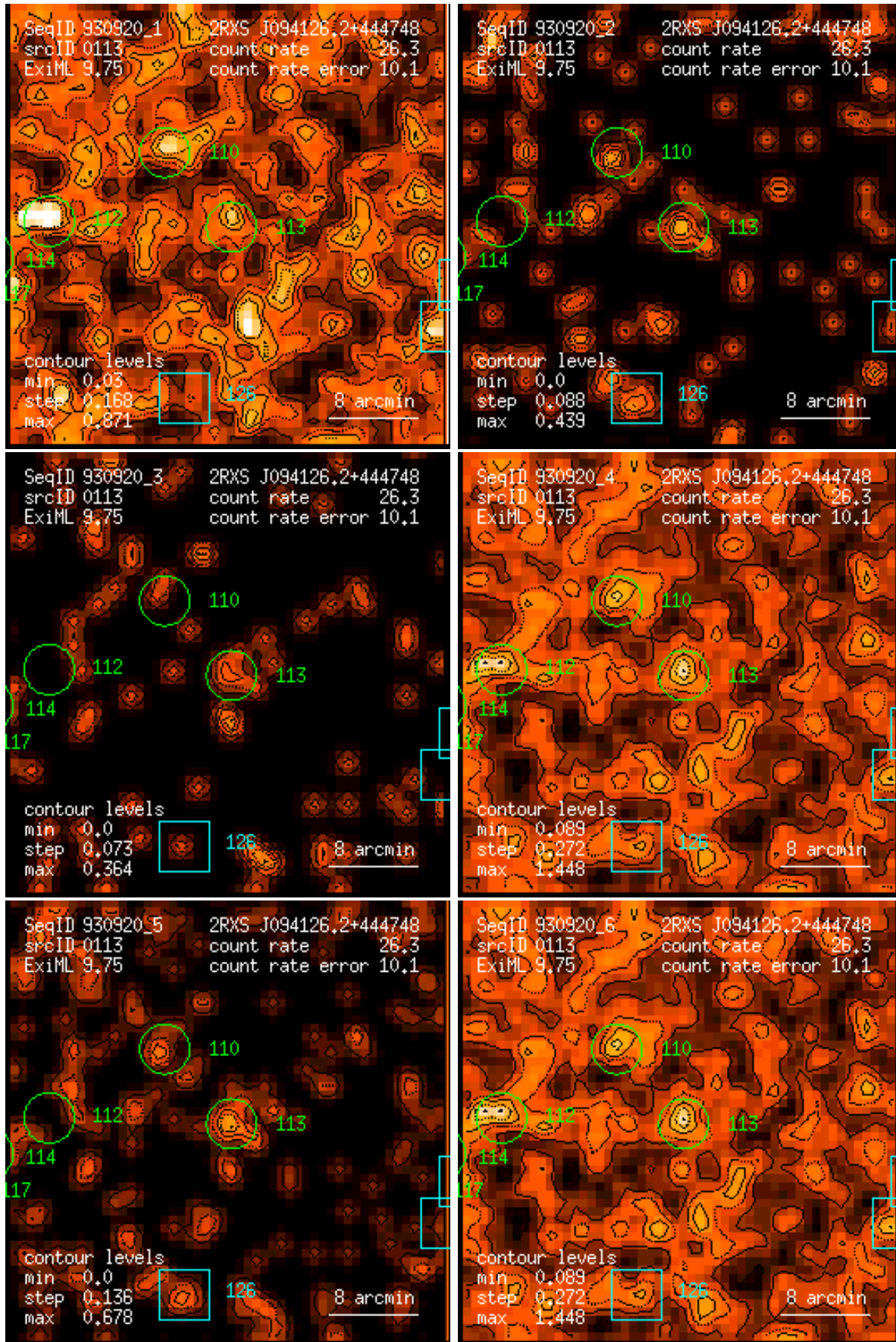
Figure 113: RASS 930920: detection 0113: band rate images, Gaussian filter: (1) PSPC channels 11 – 41, (2) 52 – 90, (3) 91 – 201, (4) 11 – 235, (5) 52 – 201, (6) 11 – 201. Broad band rates in counts/ks. Band rate contour levels in counts/ks/arcmin 2 .
