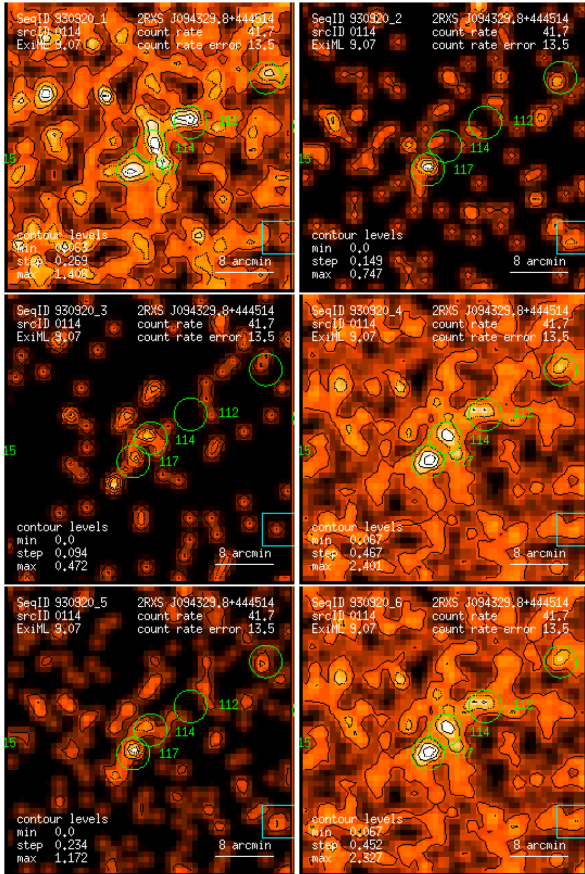
Figure 114: RASS 930920: detection 0114: band rate images, Gaussian filter: (1) PSPC channels 11 – 41, (2) 52 – 90, (3) 91 – 201, (4) 11 – 235, (5) 52 – 201, (6) 11 – 201. Broad band rates in counts/ks. Band rate contour levels in counts/ks/arcmin 2 .
