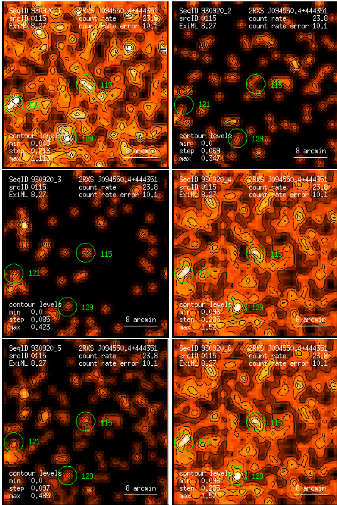
Figure 115: RASS 930920: detection 0115: band rate images, Gaussian filter: (1) PSPC channels 11 – 41, (2) 52 – 90, (3) 91 – 201, (4) 11 – 235, (5) 52 – 201, (6) 11 – 201. Broad band rates in counts/ks. Band rate contour levels in counts/ks/arcmin 2 .
