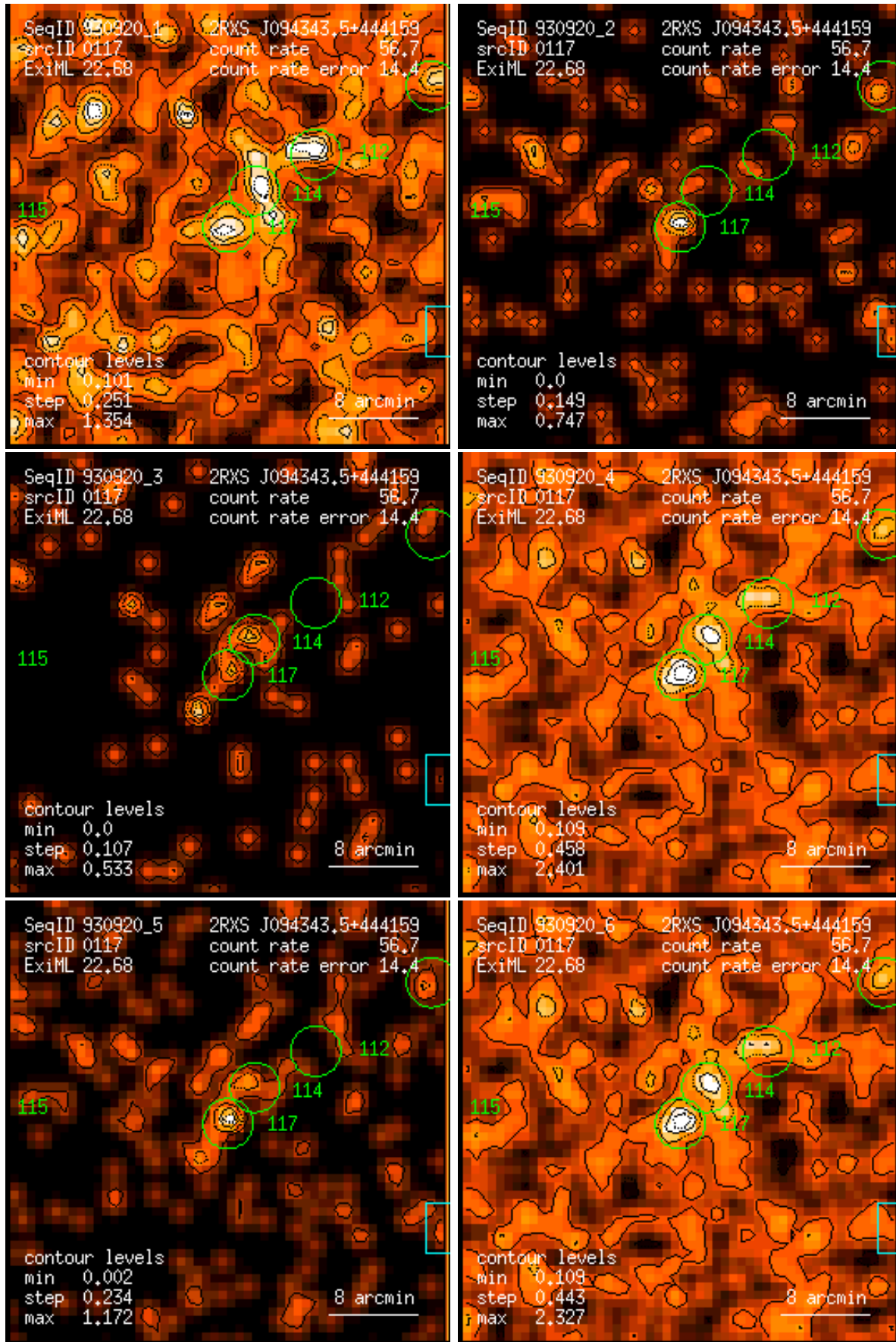
Figure 117: RASS 930920: detection 0117: band rate images, Gaussian filter: (1) PSPC channels 11 – 41, (2) 52 – 90, (3) 91 – 201, (4) 11 – 235, (5) 52 – 201, (6) 11 – 201. Broad band rates in counts/ks. Band rate contour levels in counts/ks/arcmin 2 .
