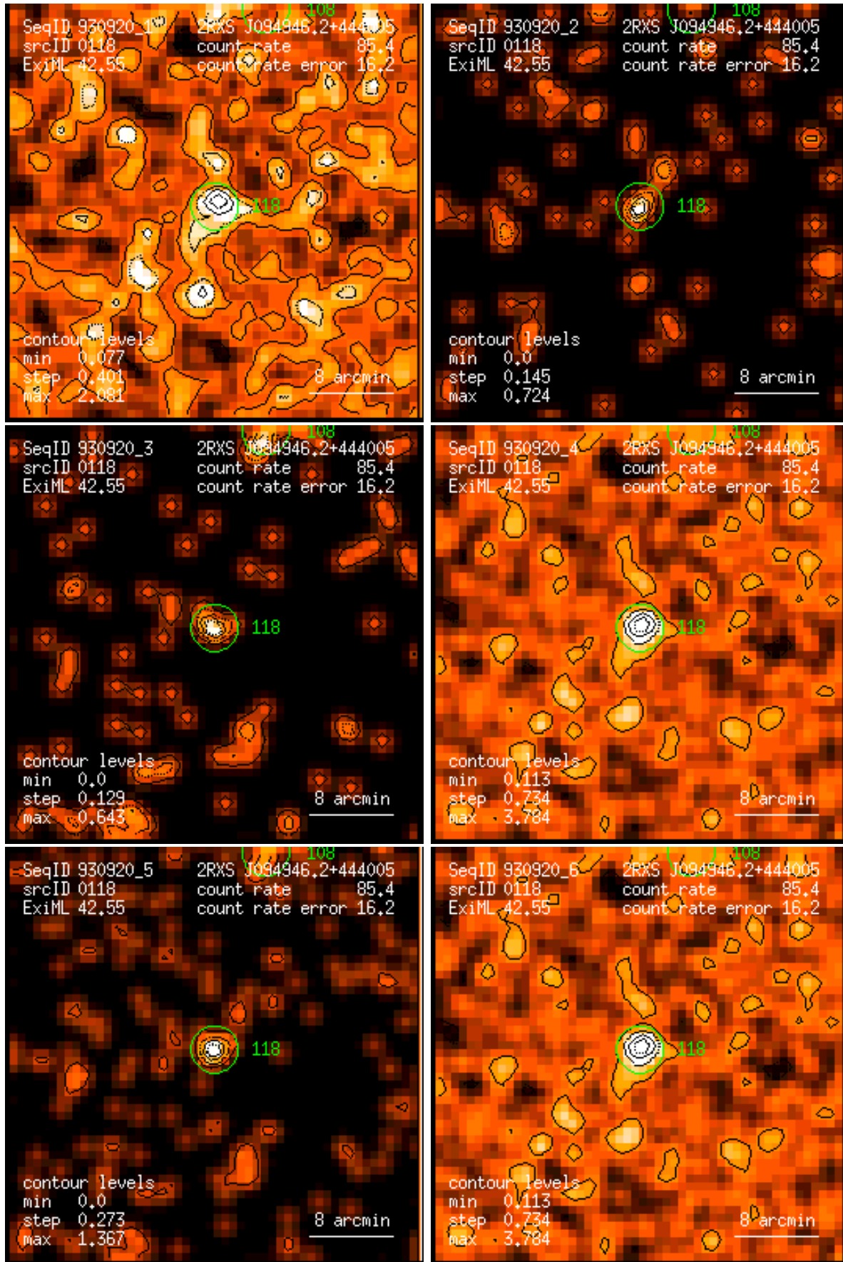
Figure 118: RASS 930920: detection 0118: band rate images, Gaussian filter: (1) PSPC channels 11 – 41, (2) 52 – 90, (3) 91 – 201, (4) 11 – 235, (5) 52 – 201, (6) 11 – 201. Broad band rates in counts/ks. Band rate contour levels in counts/ks/arcmin 2 .
