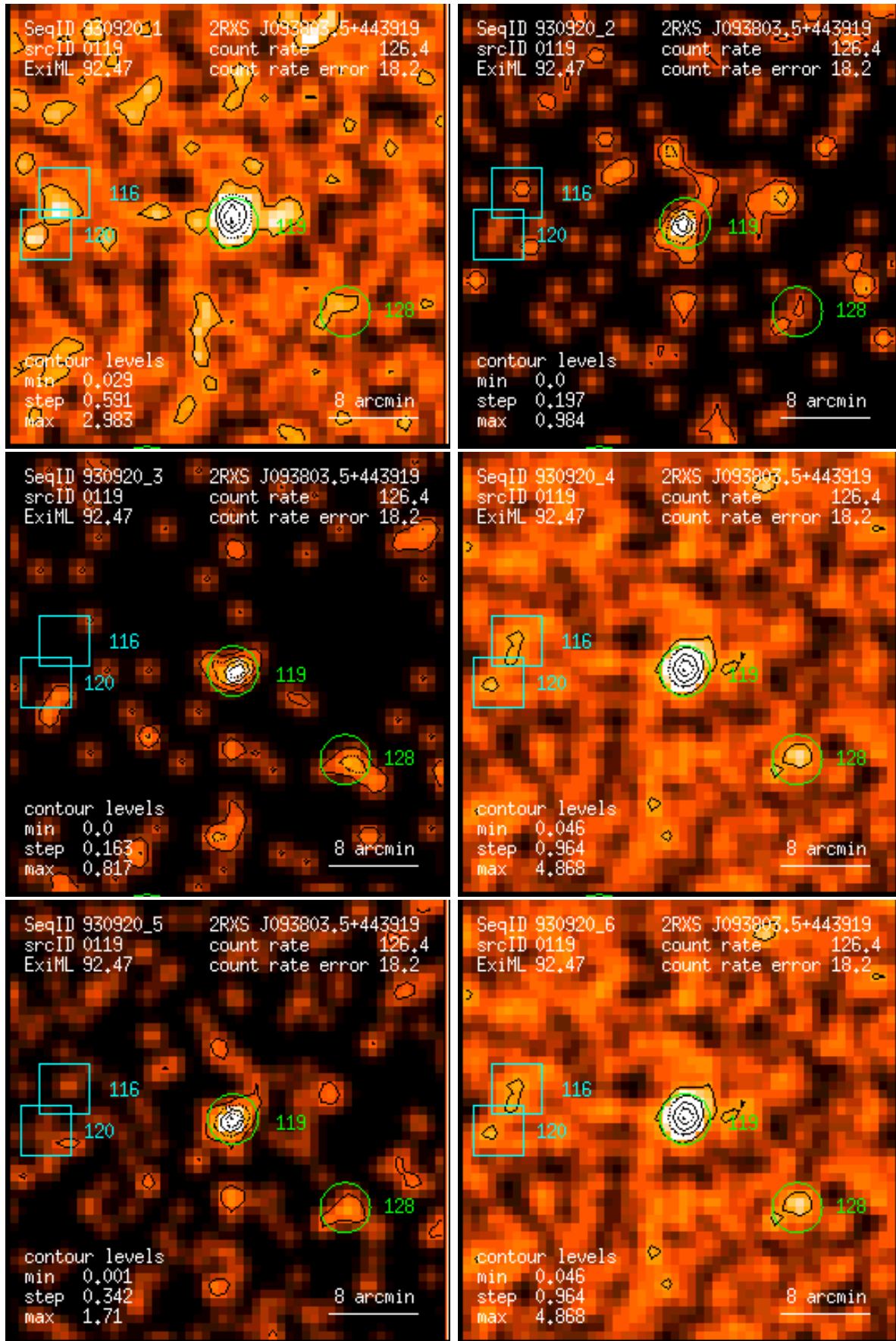
Figure 119: RASS 930920: detection 0119: band rate images, Gaussian filter: (1) PSPC channels 11 – 41, (2) 52 – 90, (3) 91 – 201, (4) 11 – 235, (5) 52 – 201, (6) 11 – 201. Broad band rates in counts/ks. Band rate contour levels in counts/ks/arcmin 2 .
