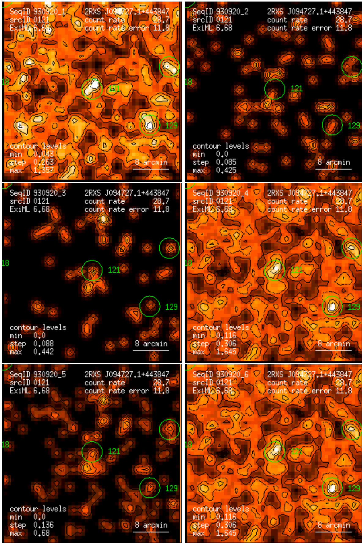
Figure 121: RASS 930920: detection 0121: band rate images, Gaussian filter: (1) PSPC channels 11 – 41, (2) 52 – 90, (3) 91 – 201, (4) 11 – 235, (5) 52 – 201, (6) 11 – 201. Broad band rates in counts/ks. Band rate contour levels in counts/ks/arcmin 2 .
