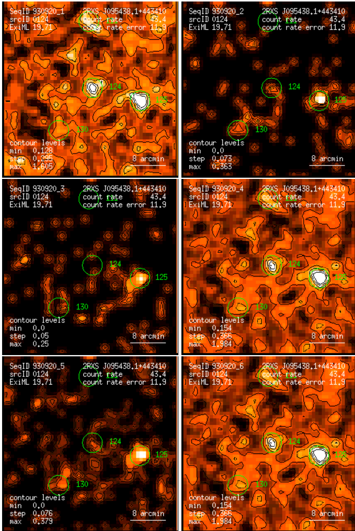
Figure 124: RASS 930920: detection 0124: band rate images, Gaussian filter: (1) PSPC channels 11 – 41, (2) 52 – 90, (3) 91 – 201, (4) 11 – 235, (5) 52 – 201, (6) 11 – 201. Broad band rates in counts/ks. Band rate contour levels in counts/ks/arcmin 2 .
