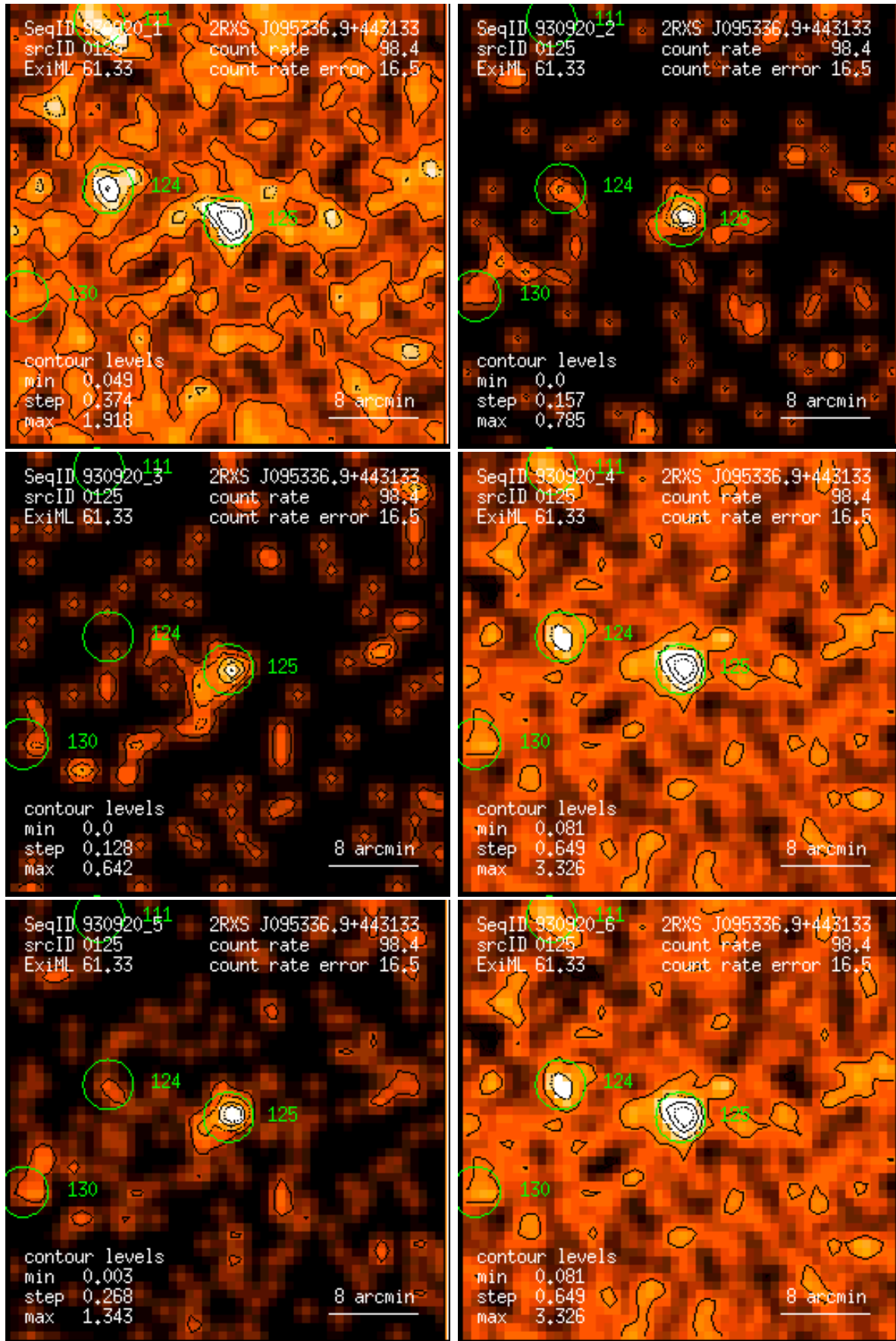
Figure 125: RASS 930920: detection 0125: band rate images, Gaussian filter: (1) PSPC channels 11 – 41, (2) 52 – 90, (3) 91 – 201, (4) 11 – 235, (5) 52 – 201, (6) 11 – 201. Broad band rates in counts/ks. Band rate contour levels in counts/ks/arcmin 2 .
