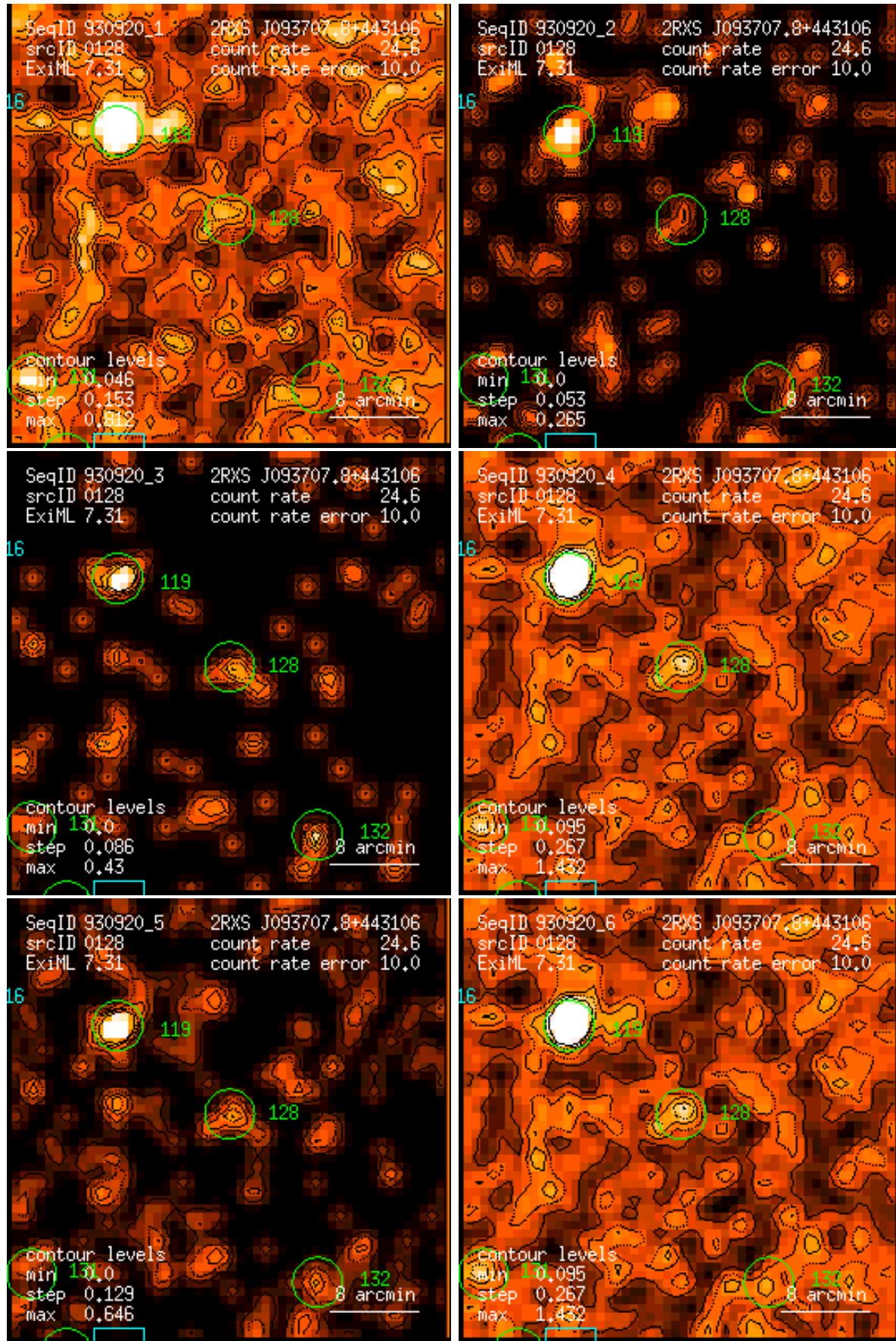
Figure 128: RASS 930920: detection 0128: band rate images, Gaussian filter: (1) PSPC channels 11 – 41, (2) 52 – 90, (3) 91 – 201, (4) 11 – 235, (5) 52 – 201, (6) 11 – 201. Broad band rates in counts/ks. Band rate contour levels in counts/ks/arcmin 2 .
