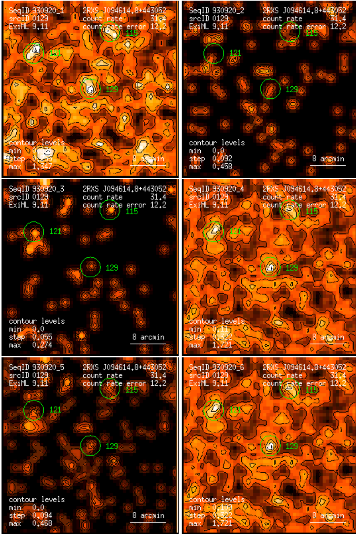
Figure 129: RASS 930920: detection 0129: band rate images, Gaussian filter: (1) PSPC channels 11 – 41, (2) 52 – 90, (3) 91 – 201, (4) 11 – 235, (5) 52 – 201, (6) 11 – 201. Broad band rates in counts/ks. Band rate contour levels in counts/ks/arcmin 2 .
