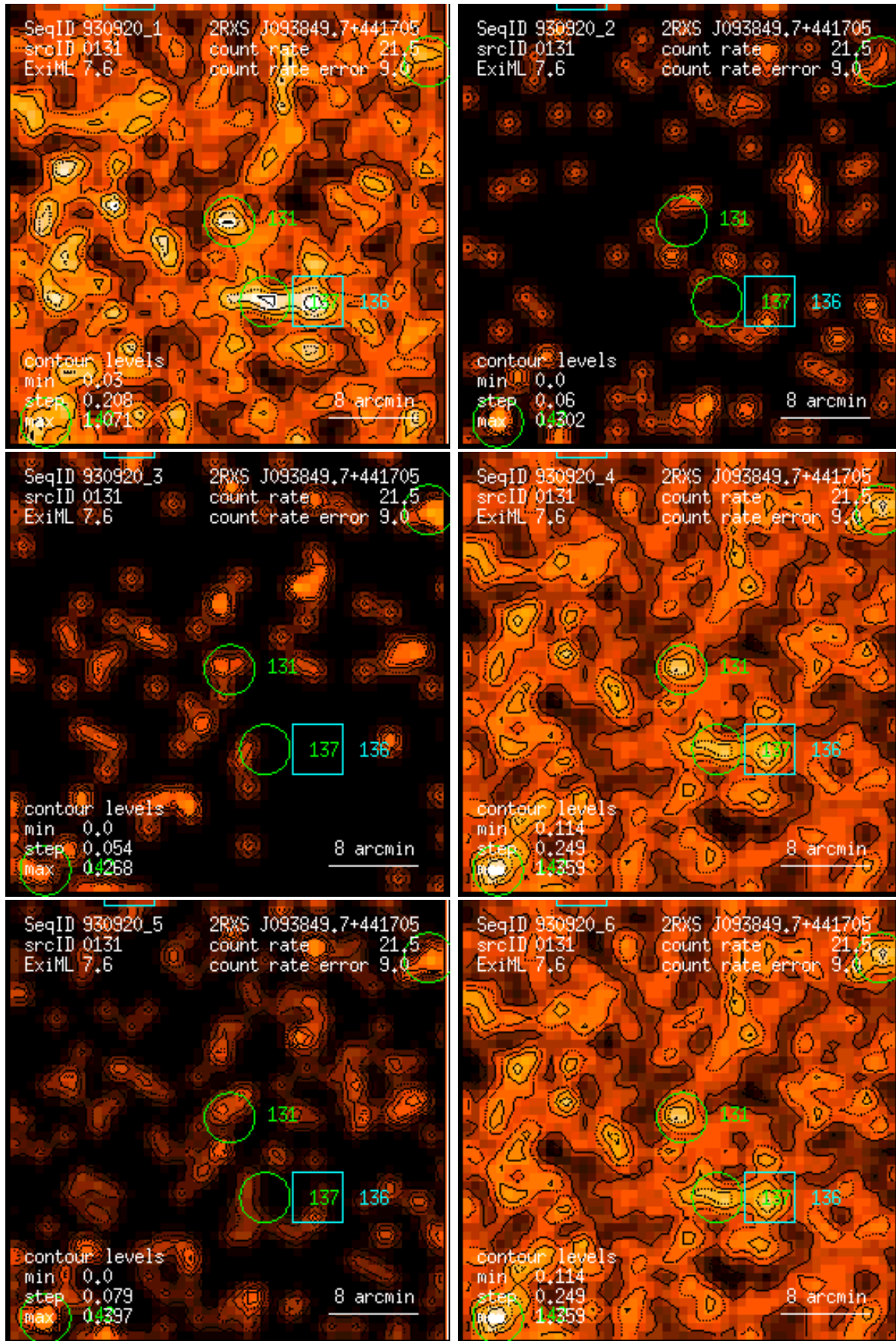
Figure 131: RASS 930920: detection 0131: band rate images, Gaussian filter: (1) PSPC channels 11 – 41, (2) 52 – 90, (3) 91 – 201, (4) 11 – 235, (5) 52 – 201, (6) 11 – 201. Broad band rates in counts/ks. Band rate contour levels in counts/ks/arcmin 2 .
