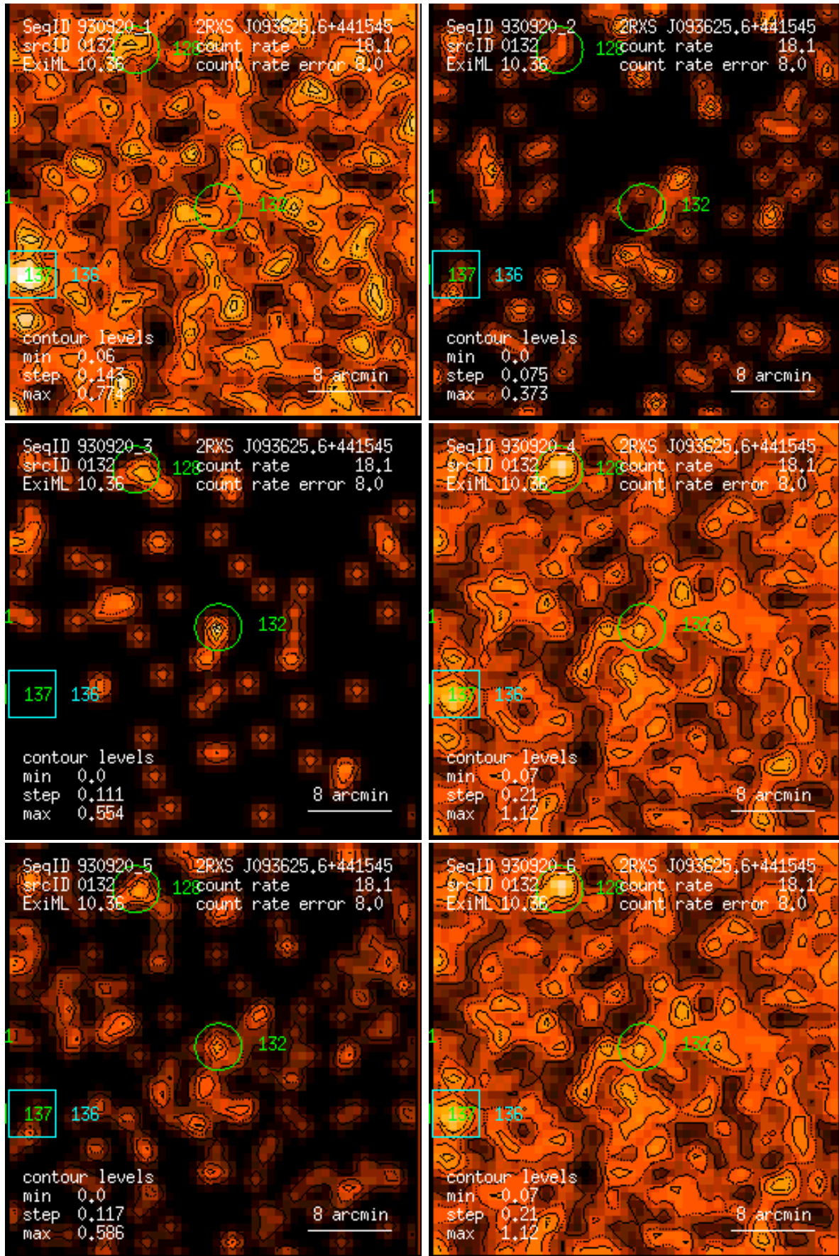
Figure 132: RASS 930920: detection 0132: band rate images, Gaussian filter: (1) PSPC channels 11 – 41, (2) 52 – 90, (3) 91 – 201, (4) 11 – 235, (5) 52 – 201, (6) 11 – 201. Broad band rates in counts/ks. Band rate contour levels in counts/ks/arcmin 2 .
