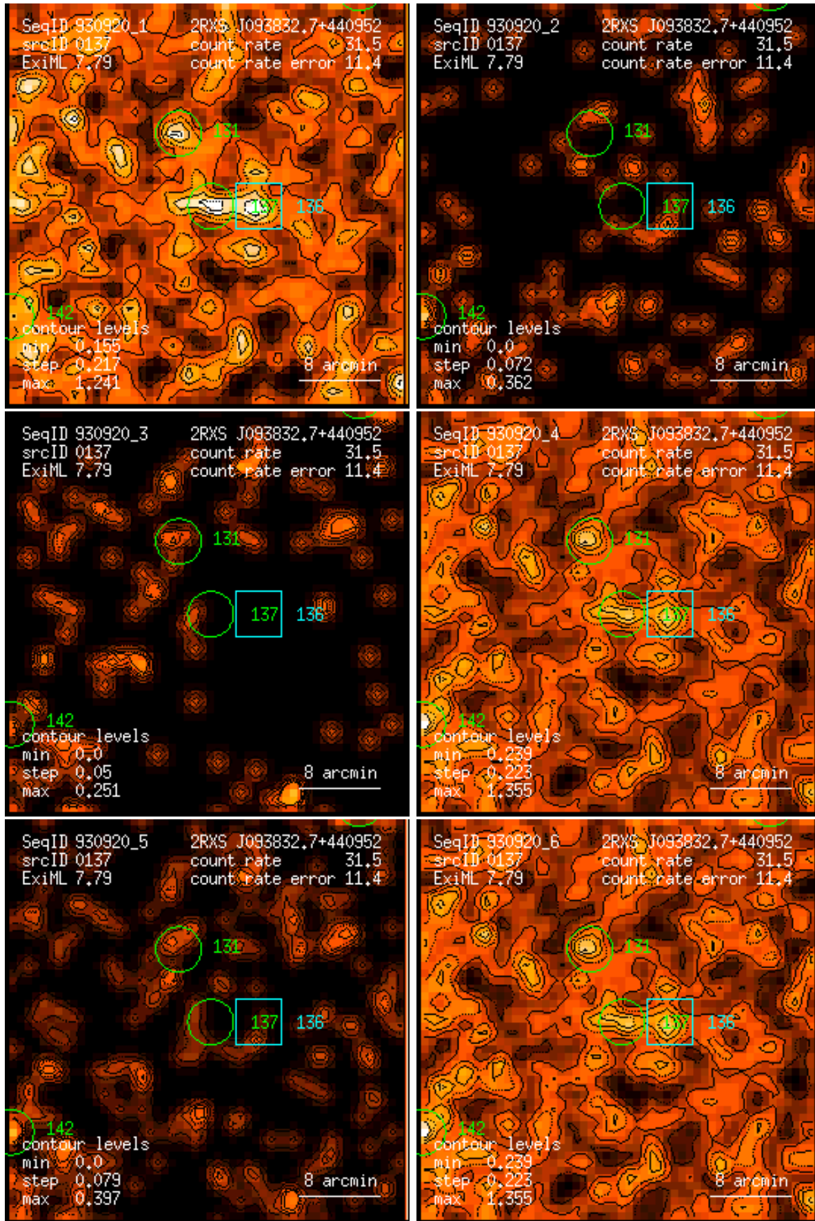
Figure 137: RASS 930920: detection 0137: band rate images, Gaussian filter: (1) PSPC channels 11 – 41, (2) 52 – 90, (3) 91 – 201, (4) 11 – 235, (5) 52 – 201, (6) 11 – 201. Broad band rates in counts/ks. Band rate contour levels in counts/ks/arcmin 2 .
