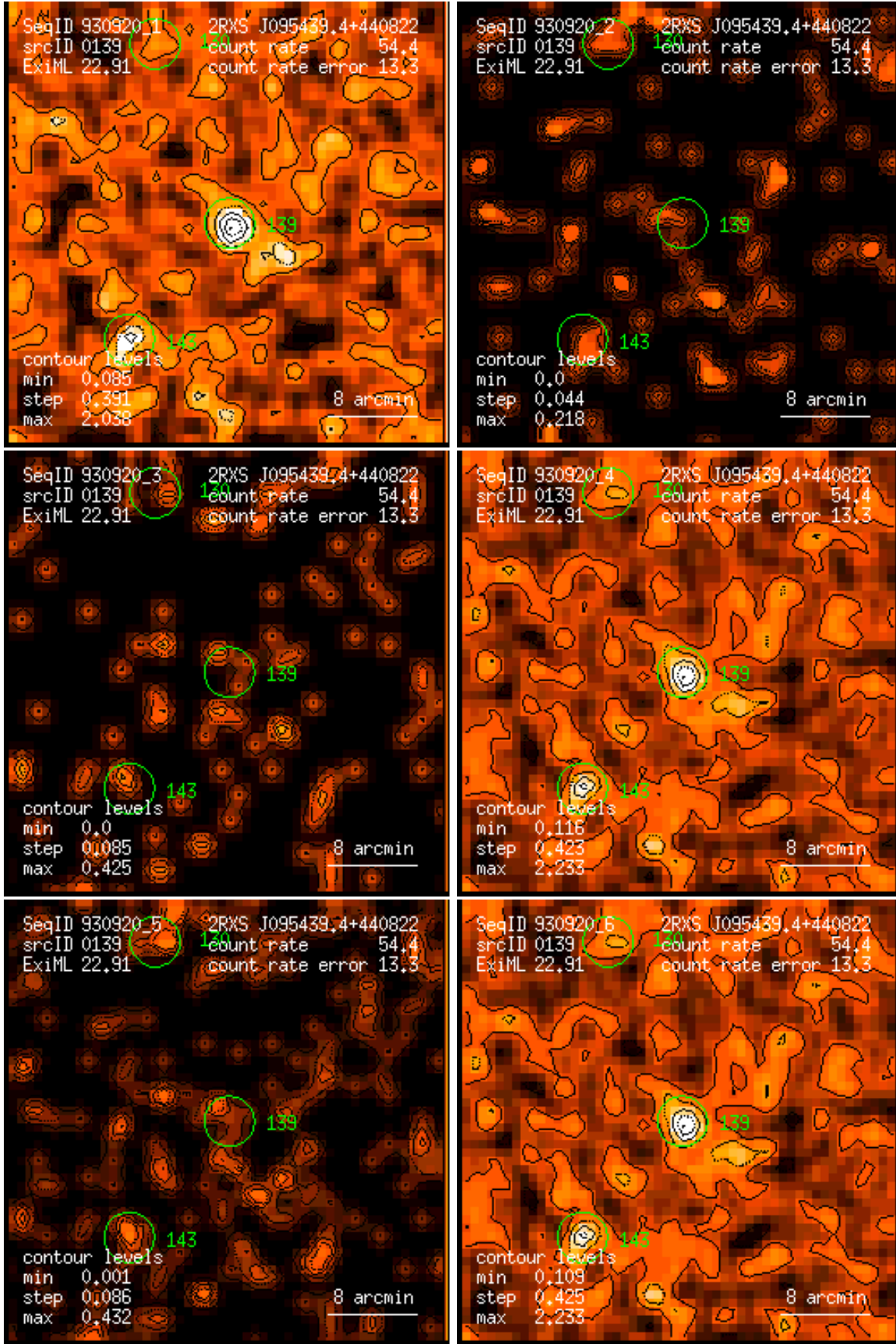
Figure 139: RASS 930920: detection 0139: band rate images, Gaussian filter: (1) PSPC channels 11 – 41, (2) 52 – 90, (3) 91 – 201, (4) 11 – 235, (5) 52 – 201, (6) 11 – 201. Broad band rates in counts/ks. Band rate contour levels in counts/ks/arcmin 2 .
