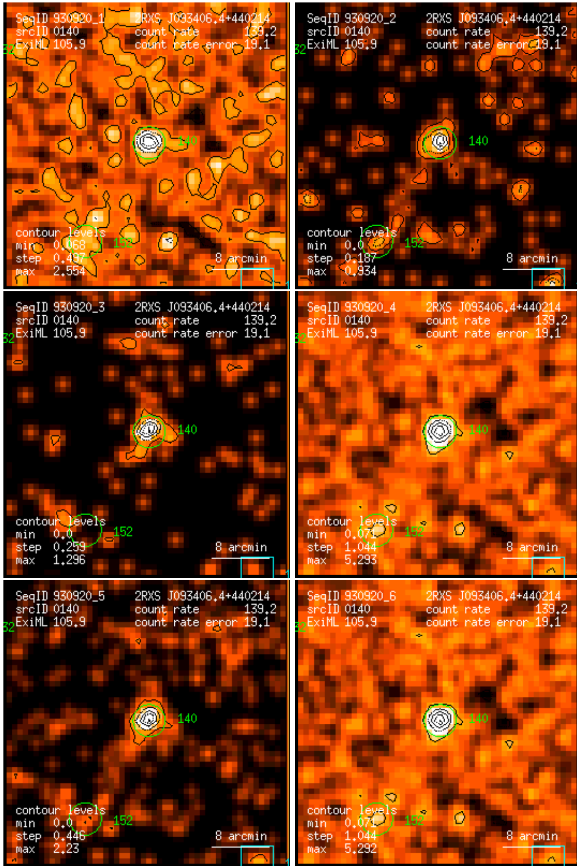
Figure 140: RASS 930920: detection 0140: band rate images, Gaussian filter: (1) PSPC channels 11 – 41, (2) 52 – 90, (3) 91 – 201, (4) 11 – 235, (5) 52 – 201, (6) 11 – 201. Broad band rates in counts/ks. Band rate contour levels in counts/ks/arcmin 2 .
