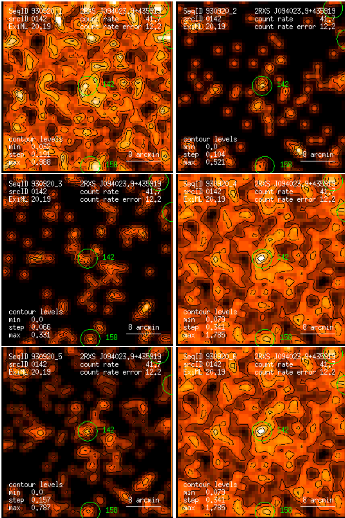
Figure 142: RASS 930920: detection 0142: band rate images, Gaussian filter: (1) PSPC channels 11 – 41, (2) 52 – 90, (3) 91 – 201, (4) 11 – 235, (5) 52 – 201, (6) 11 – 201. Broad band rates in counts/ks. Band rate contour levels in counts/ks/arcmin 2 .
