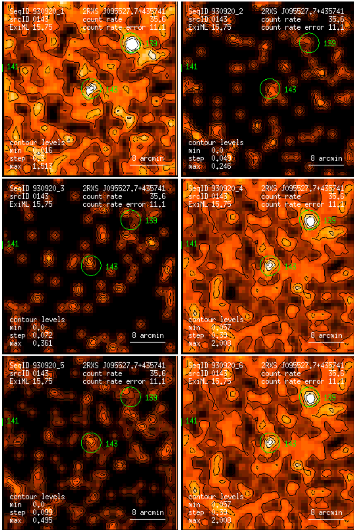
Figure 143: RASS 930920: detection 0143: band rate images, Gaussian filter: (1) PSPC channels 11 – 41, (2) 52 – 90, (3) 91 – 201, (4) 11 – 235, (5) 52 – 201, (6) 11 – 201. Broad band rates in counts/ks. Band rate contour levels in counts/ks/arcmin 2 .
