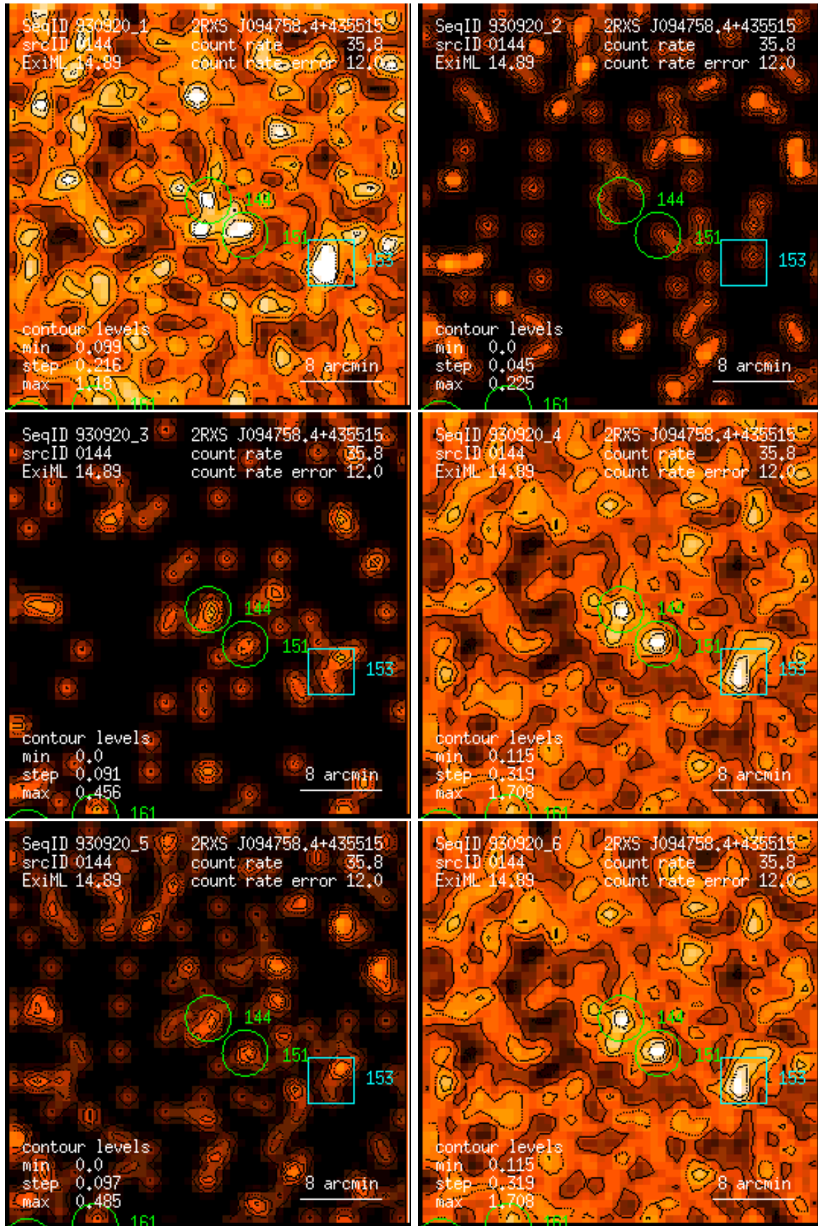
Figure 144: RASS 930920: detection 0144: band rate images, Gaussian filter: (1) PSPC channels 11 – 41, (2) 52 – 90, (3) 91 – 201, (4) 11 – 235, (5) 52 – 201, (6) 11 – 201. Broad band rates in counts/ks. Band rate contour levels in counts/ks/arcmin 2 .
