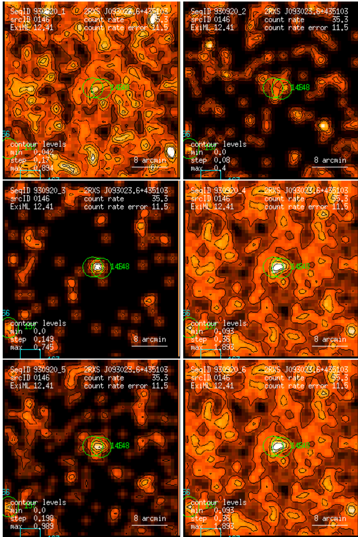
Figure 146: RASS 930920: detection 0146: band rate images, Gaussian filter: (1) PSPC channels 11 – 41, (2) 52 – 90, (3) 91 – 201, (4) 11 – 235, (5) 52 – 201, (6) 11 – 201. Broad band rates in counts/ks. Band rate contour levels in counts/ks/arcmin 2 .
