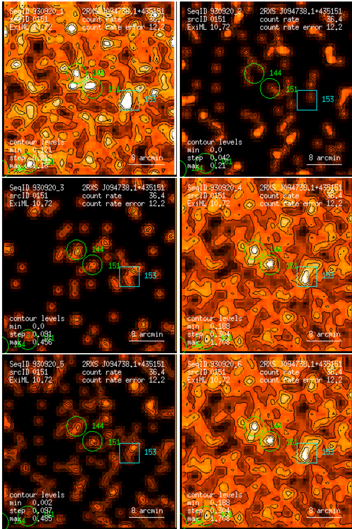
Figure 151: RASS 930920: detection 0151: band rate images, Gaussian filter: (1) PSPC channels 11 – 41, (2) 52 – 90, (3) 91 – 201, (4) 11 – 235, (5) 52 – 201, (6) 11 – 201. Broad band rates in counts/ks. Band rate contour levels in counts/ks/arcmin 2 .
