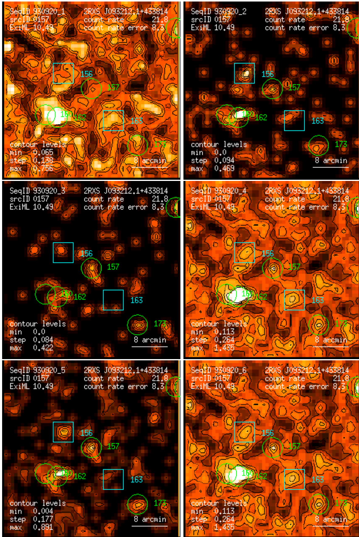
Figure 157: RASS 930920: detection 0157: band rate images, Gaussian filter: (1) PSPC channels 11 – 41, (2) 52 – 90, (3) 91 – 201, (4) 11 – 235, (5) 52 – 201, (6) 11 – 201. Broad band rates in counts/ks. Band rate contour levels in counts/ks/arcmin 2 .
