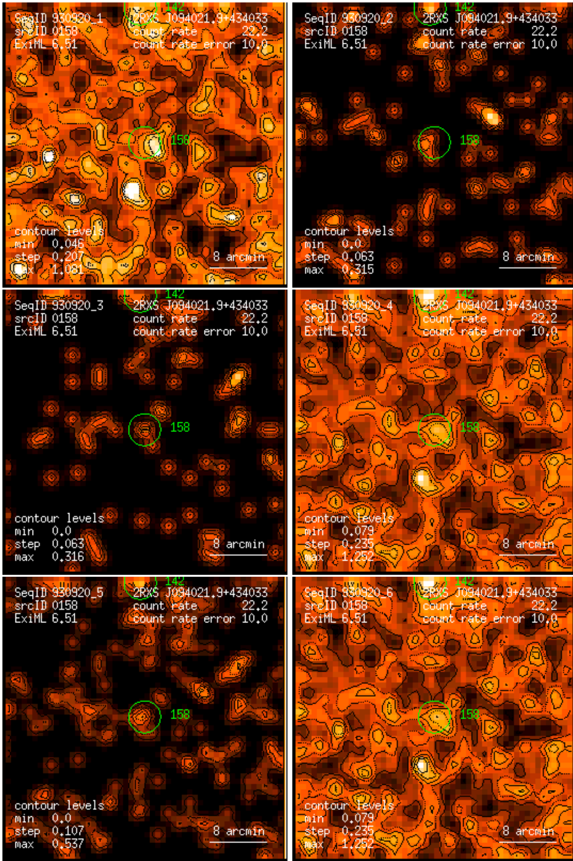
Figure 158: RASS 930920: detection 0158: band rate images, Gaussian filter: (1) PSPC channels 11 – 41, (2) 52 – 90, (3) 91 – 201, (4) 11 – 235, (5) 52 – 201, (6) 11 – 201. Broad band rates in counts/ks. Band rate contour levels in counts/ks/arcmin 2 .
