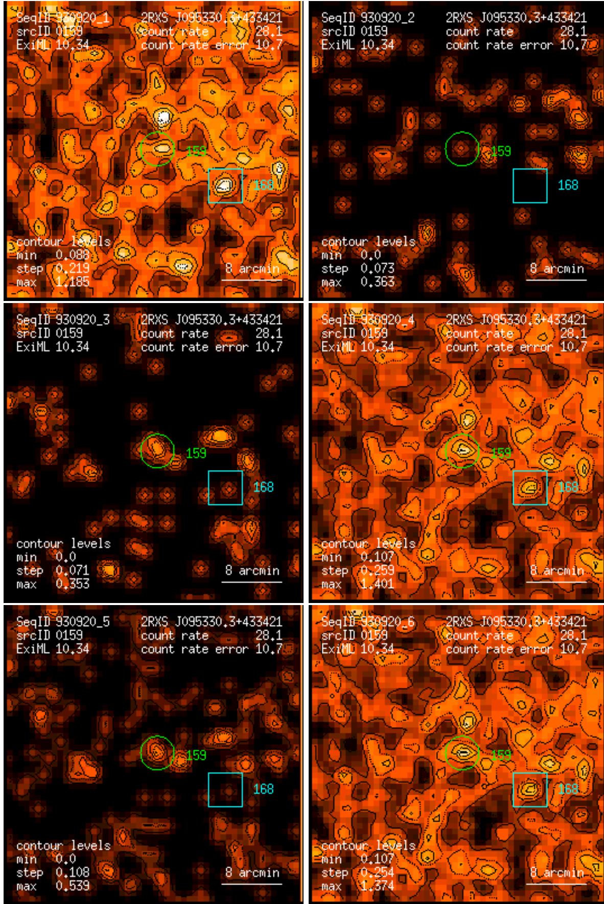
Figure 159: RASS 930920: detection 0159: band rate images, Gaussian filter: (1) PSPC channels 11 – 41, (2) 52 – 90, (3) 91 – 201, (4) 11 – 235, (5) 52 – 201, (6) 11 – 201. Broad band rates in counts/ks. Band rate contour levels in counts/ks/arcmin 2 .
