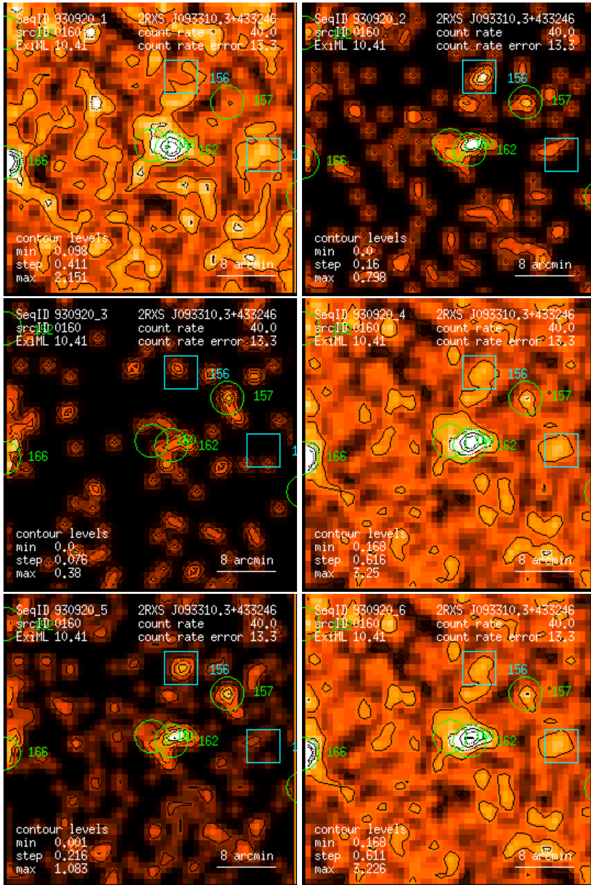
Figure 160: RASS 930920: detection 0160: band rate images, Gaussian filter: (1) PSPC channels 11 – 41, (2) 52 – 90, (3) 91 – 201, (4) 11 – 235, (5) 52 – 201, (6) 11 – 201. Broad band rates in counts/ks. Band rate contour levels in counts/ks/arcmin 2 .
