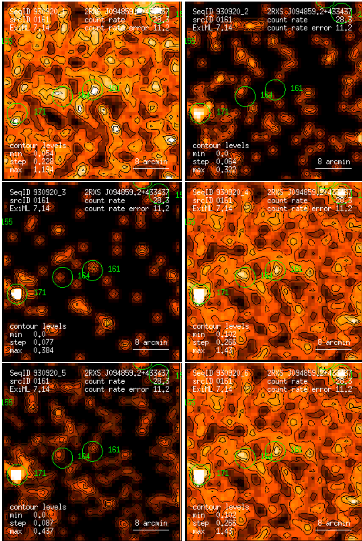
Figure 161: RASS 930920: detection 0161: band rate images, Gaussian filter: (1) PSPC channels 11 – 41, (2) 52 – 90, (3) 91 – 201, (4) 11 – 235, (5) 52 – 201, (6) 11 – 201. Broad band rates in counts/ks. Band rate contour levels in counts/ks/arcmin 2 .
