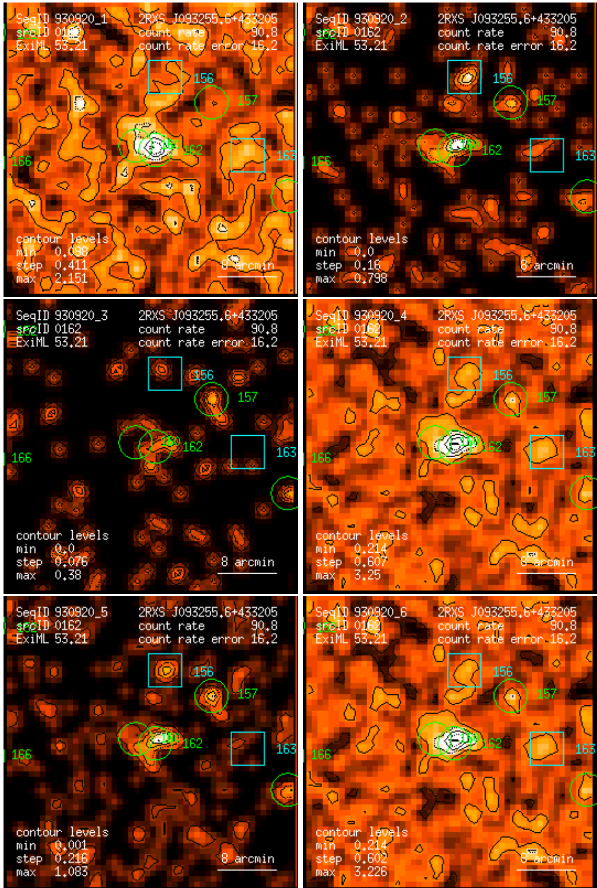
Figure 162: RASS 930920: detection 0162: band rate images, Gaussian filter: (1) PSPC channels 11 – 41, (2) 52 – 90, (3) 91 – 201, (4) 11 – 235, (5) 52 – 201, (6) 11 – 201. Broad band rates in counts/ks. Band rate contour levels in counts/ks/arcmin 2 .
