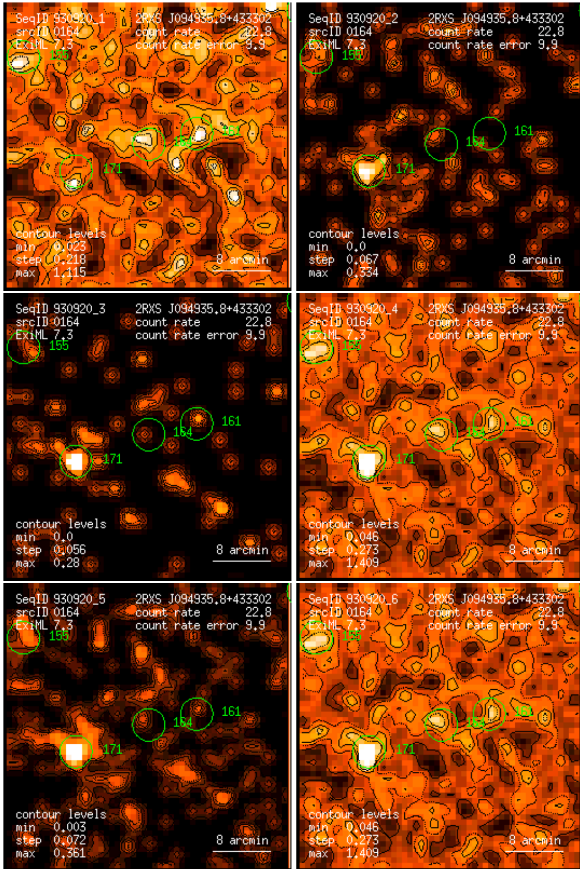
Figure 164: RASS 930920: detection 0164: band rate images, Gaussian filter: (1) PSPC channels 11 – 41, (2) 52 – 90, (3) 91 – 201, (4) 11 – 235, (5) 52 – 201, (6) 11 – 201. Broad band rates in counts/ks. Band rate contour levels in counts/ks/arcmin 2 .
