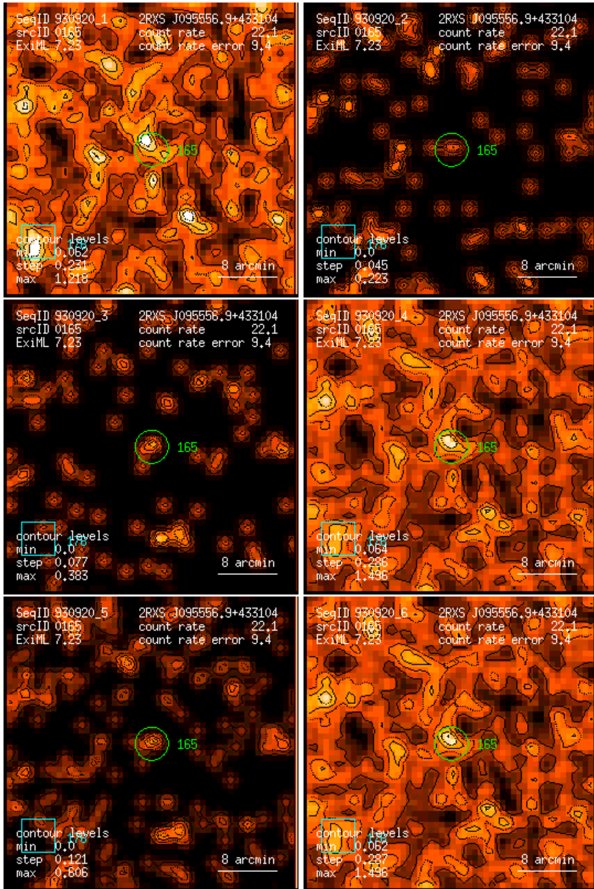
Figure 165: RASS 930920: detection 0165: band rate images, Gaussian filter: (1) PSPC channels 11 – 41, (2) 52 – 90, (3) 91 – 201, (4) 11 – 235, (5) 52 – 201, (6) 11 – 201. Broad band rates in counts/ks. Band rate contour levels in counts/ks/arcmin 2 .
