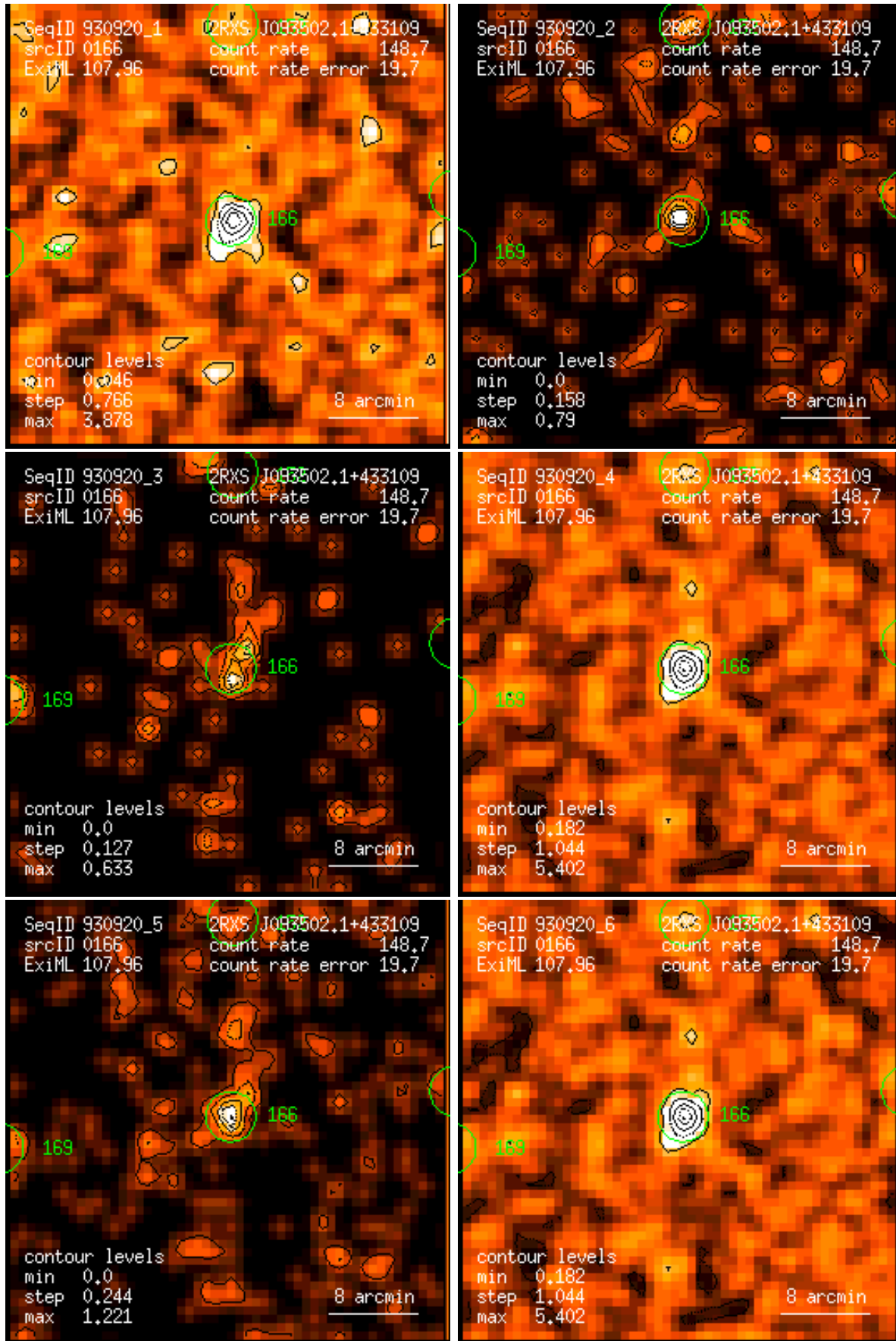
Figure 166: RASS 930920: detection 0166: band rate images, Gaussian filter: (1) PSPC channels 11 – 41, (2) 52 – 90, (3) 91 – 201, (4) 11 – 235, (5) 52 – 201, (6) 11 – 201. Broad band rates in counts/ks. Band rate contour levels in counts/ks/arcmin 2 .
