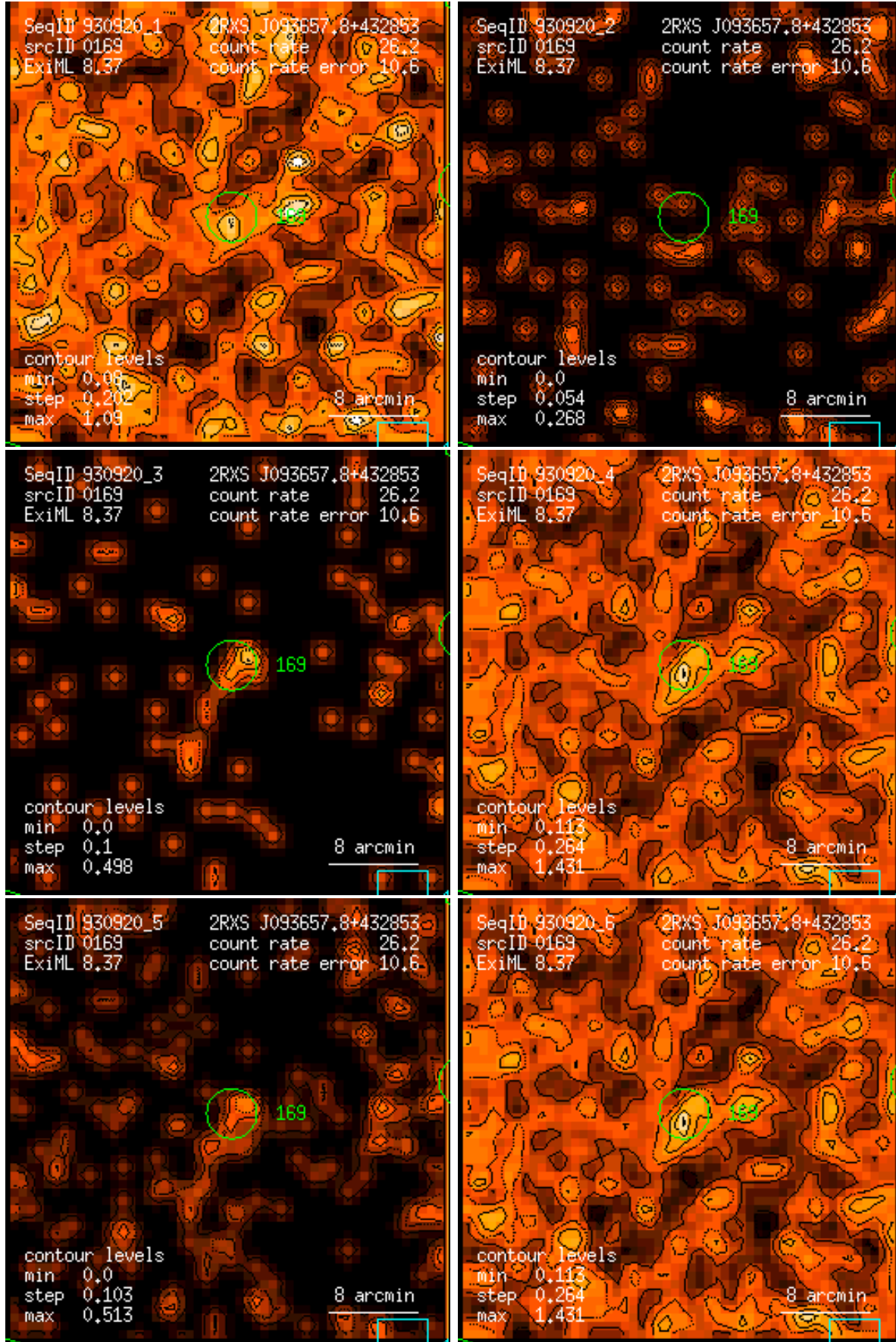
Figure 169: RASS 930920: detection 0169: band rate images, Gaussian filter: (1) PSPC channels 11 – 41, (2) 52 – 90, (3) 91 – 201, (4) 11 – 235, (5) 52 – 201, (6) 11 – 201. Broad band rates in counts/ks. Band rate contour levels in counts/ks/arcmin 2 .
