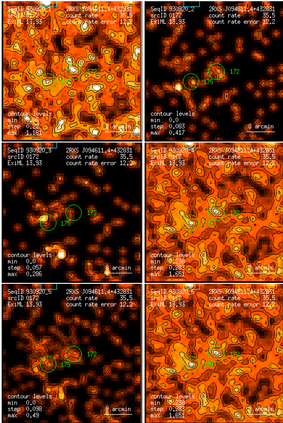
Figure 172: RASS 930920: detection 0172: band rate images, Gaussian filter: (1) PSPC channels 11 – 41, (2) 52 – 90, (3) 91 – 201, (4) 11 – 235, (5) 52 – 201, (6) 11 – 201. Broad band rates in counts/ks. Band rate contour levels in counts/ks/arcmin 2 .
