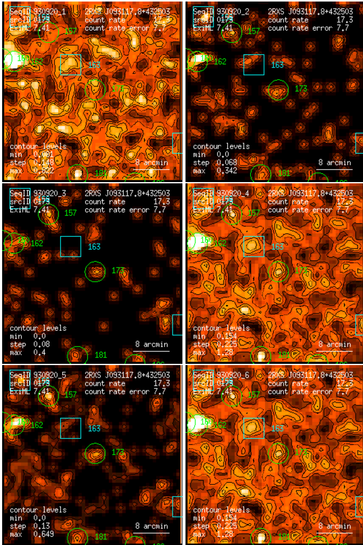
Figure 173: RASS 930920: detection 0173: band rate images, Gaussian filter: (1) PSPC channels 11 – 41, (2) 52 – 90, (3) 91 – 201, (4) 11 – 235, (5) 52 – 201, (6) 11 – 201. Broad band rates in counts/ks. Band rate contour levels in counts/ks/arcmin 2 .
