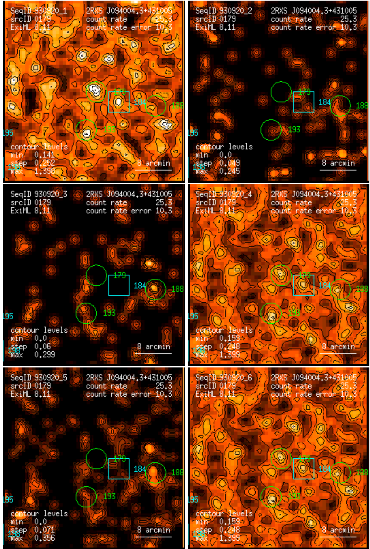
Figure 179: RASS 930920: detection 0179: band rate images, Gaussian filter: (1) PSPC channels 11 – 41, (2) 52 – 90, (3) 91 – 201, (4) 11 – 235, (5) 52 – 201, (6) 11 – 201. Broad band rates in counts/ks. Band rate contour levels in counts/ks/arcmin 2 .
