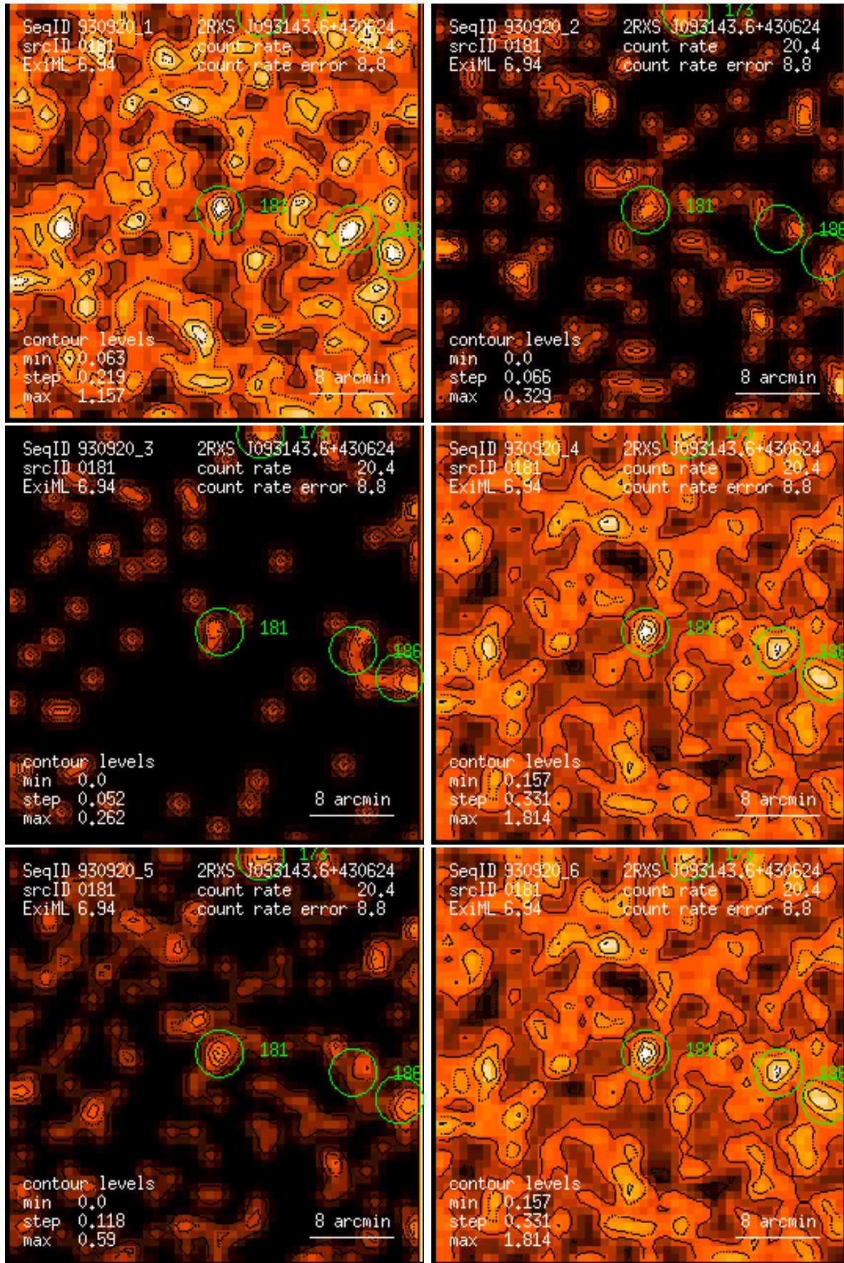
Figure 181: RASS 930920: detection 0181: band rate images, Gaussian filter: (1) PSPC channels 11 – 41, (2) 52 – 90, (3) 91 – 201, (4) 11 – 235, (5) 52 – 201, (6) 11 – 201. Broad band rates in counts/ks. Band rate contour levels in counts/ks/arcmin 2 .
