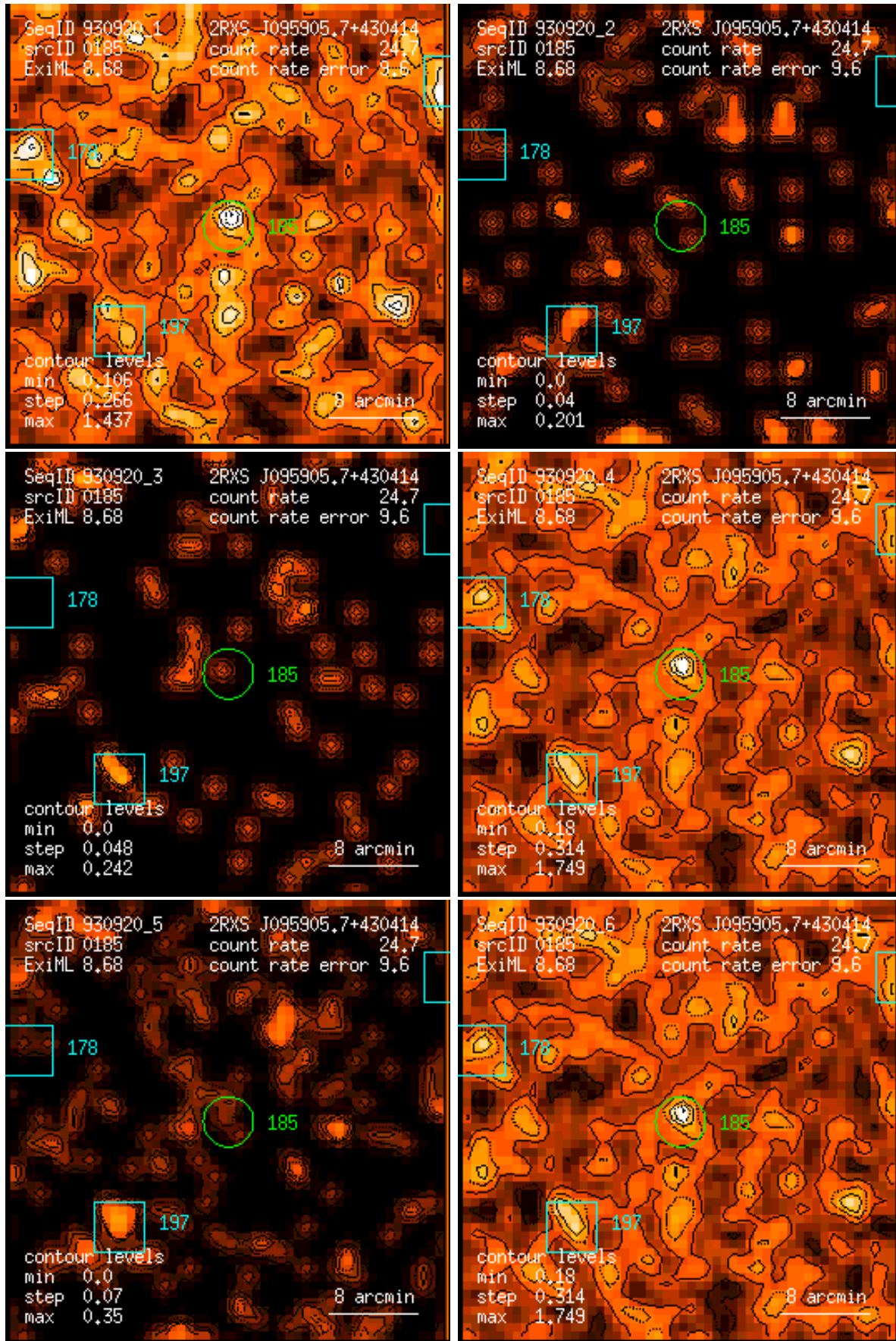
Figure 185: RASS 930920: detection 0185: band rate images, Gaussian filter: (1) PSPC channels 11 – 41, (2) 52 – 90, (3) 91 – 201, (4) 11 – 235, (5) 52 – 201, (6) 11 – 201. Broad band rates in counts/ks. Band rate contour levels in counts/ks/arcmin 2 .
